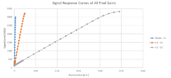
Fig. 9. Signal Response Curves for the Diode, C0 and C1
