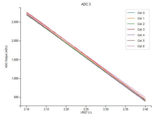
Fig. 8. Example ADC traces for a nominal PGA gain of 6
