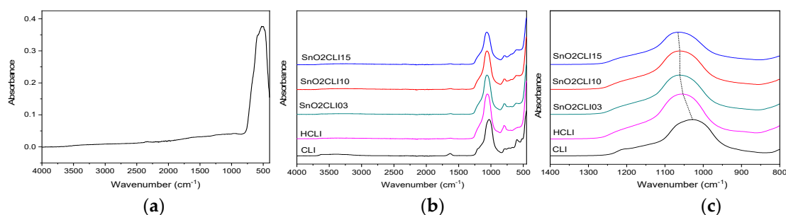
Figure 7. Attenuated total reflection (ATR)-FTIR spectra of (a) \text{SnO}_2 and (b) \text{SnO}_2 -containing clinoptilolite. In (c) a closer range ( 1400\text{--}800\text{ cm}^{-1} ) is shown.
