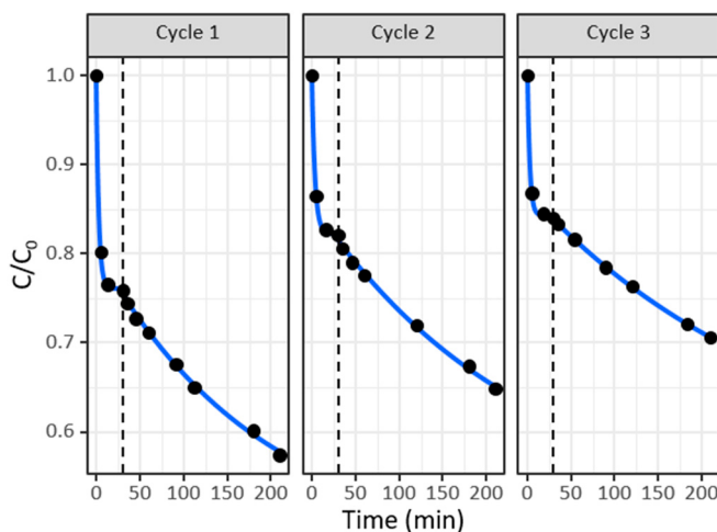
Figure 12. Reusability of the photocatalyst SnO 2 CLI25 in photodegradation of MB. The illumination part of the reaction, right of the dashed line, is fitted to Equation. 1 with a blue solid line. Reaction conditions: V = 50 \text{ cm}^3 , \text{O}_2 \text{ flow} = 25 \text{ cm}^3 \text{ min}^{-1} , T = 22 \text{ }^\circ\text{C} , C_0 = 10 \text{ mg dm}^{-3} , m_{\text{cat}} = 10 \text{ mg} .
