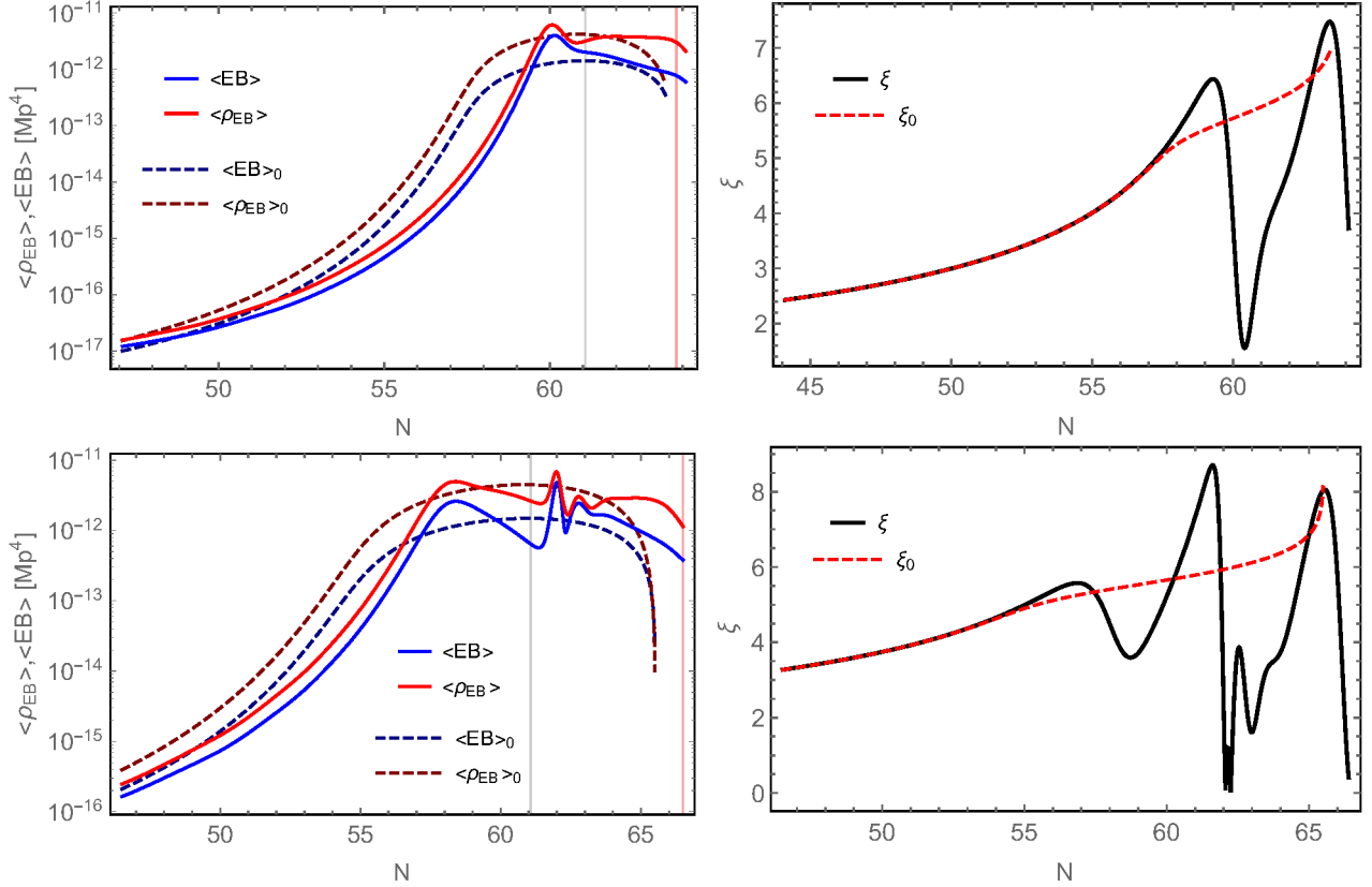
Figure 6: Top: 1/f = 20 . Bottom: 1/f = 25 . Left panels show the numerical results of \rho_{EB} and \langle \vec{E} \vec{B} \rangle (solid lines) compared to their analytical estimate (13), (14) (dashed lines). The vertical lines refer to the end of inflation in absence of backreaction (black line) and for the full numerical analysis (red line). Right panels show the oscillatory behaviour of the \xi parameter (solid black line) compared to its analytical result coming from the solution of the inflaton equation of motion when the gauge field backreaction is given by (13) (dashed red line). For better visibility, we display only the last \sim 20 e-folds of inflation.
