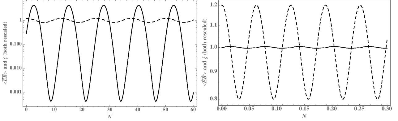
Figure 3: Left: Numerically computed, and rescaled, response of \langle \vec{E}\vec{B} \rangle with significant lag (solid black) for a harmonic perturbation of \xi with near-critical frequency \omega_N \sim \omega_N^* (dashed black). Right: For much larger frequencies the response averages out to zero. We chose \bar{\xi} = 5 and the oscillation amplitude \Delta\xi = 1 .
