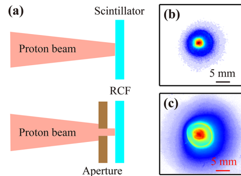
FIG. 2. (a) Schematic of the experimental setup at NDCX-II. A scintillator was placed at the focal plane of the proton beam, and a gated intensified CCD camera was used to capture the light emitted from the scintillator when struck by the proton bunch. RCF HD-v2 films were then located in the same location and were irradiated by either an apertured proton beam (2 mm diameter) or the full beam (2.7 mm diameter). Examples of the dose distributions are shown in (b) and (c) for the full beam measured in situ with the scintillator (b) and by RCF ex situ (c).
