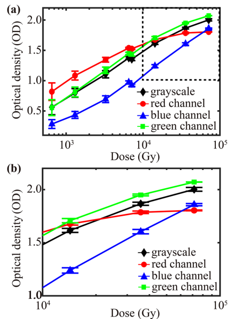
FIG. 3. (a) Dose response curves of separate RGB channels and the grayscale for GaFChromic RCF HD-v2 with LDR mode. The vertical error bars indicate the standard deviation for each dose. (b) Magnified view of the black dotted zone of very high doses in (a).
