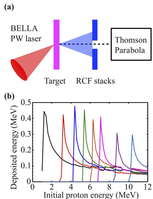
FIG. 5. (a) Schematic of the experimental setup for laser driven ion acceleration at BELLA center. The BELLA PW laser pulse irradiates the target (a few micrometer thick Ti foils) at an oblique incidence angle of 45^\circ . Protons are characterized with a Thomson parabola and RCF stacks. (b) RCF response functions for the stacks used in the experiments, which consists of 6 layers of HD-v2 followed by 2 layers of MD-v3. Here, the MD-v3 is calibrated by Ref. 34.
