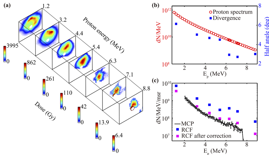
FIG. 6. (a) Three-dimensional proton spectrum for a 5 \mu\text{m} thick titanium foil irradiated by the BELLA PW laser. Each slice presents a RCF layer measurement that was normalized to the local dose maximum. The slices are plotted at a proton energy corresponding to the proton Bragg peak energy, and individual doses are indicated in the color bar below. The corresponding proton beam divergence (blue squares) and reconstructed space-integrated proton spectra (red circles) are shown in (b). The comparison between the measurements from the RCF stack (squares) and the TP spectrometer along with MCP (black curve) is shown in (c). The blue squares represent the derived energy distribution for the most energetic protons based on the reconstructed space-integrated proton spectra and the proton beam divergence, and magenta squares with correction for the detector position in the TP spectrometer.
