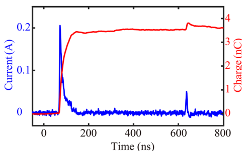
FIG. 1. Example of a proton pulse (1 MeV) from NDCX-II with current profile (blue) and integrated charge (red) from a fast Faraday cup. The peak at 636 ns is from \text{H}_2^+ ions. The proton pulse length was 10.12 \pm 1.29 ns (FWHM).
