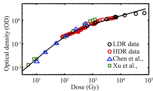
FIG. 4. Double logarithmic dose response curve in the grayscale for the full dynamic range of 3 orders of magnitudes at NDCX-II, including both LDR (black circles) and HDR (red circles) results. The black curve shows the best fitted results with a polynomial function, which is well aligned with the previous calibration results (blue triangles and green squares) 22,31 for doses below 1 kGy.
