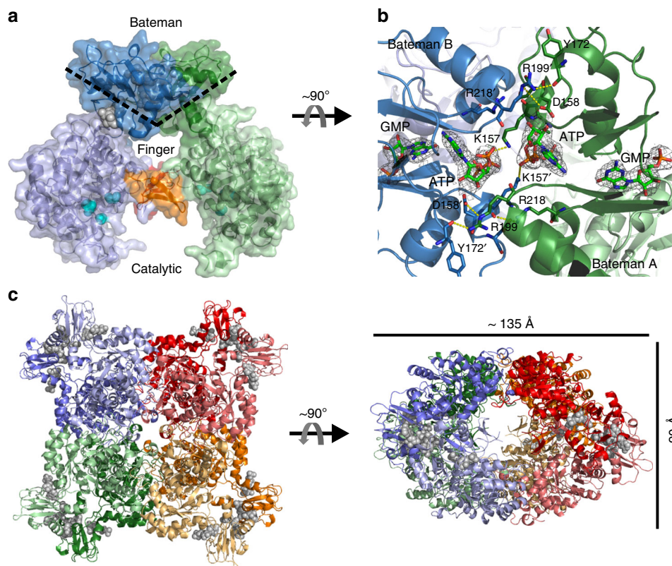
Fig. 7 Quaternary structure of TbIMPDH-ATP1/GMP2. a Relative orientation of two TbIMPDH monomers located in the ASU, estimated by the approximate angle spanned by the two beta sheets of the CBS motifs in each Bateman domain, as indicated by the dashed line. The finger domains are highlighted (orange/red), the catalytic residues (cyan), and the bound nucleotides (gray) are shown as spheres. b Detailed view on the interface formed by the adjacent Bateman domains (green/blue, cartoon representation) within the TbIMPDH dimer. Residues involved in the dimer interaction (yellow dashes) and ATP/GMP molecules are shown as sticks. The displayed 2F_o - F_c -electron density of ATP and GMP is countered at 1.0 sigma. c Cartoon representation of the octamer assembly of TbIMPDH monomers, as observed within the in cellulo crystals and corresponding space group, in different views rotated by 90^\circ . Four dimers are forming an octamer around the 4-fold symmetry axis. The dimeric building blocks observed within the ASU are individually colored. Bound nucleotides are shown in a gray spheres representation.
