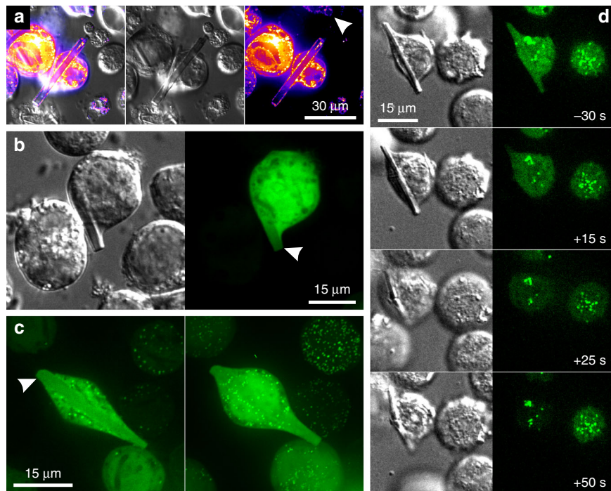
Fig. 3 Localization of TbIMPDH crystals within cellular compartments. a Co-infection of Sf9 cells with recombinant baculoviruses (rBVs) containing the genes for TbIMPDH and Pex3-mCherry fusion protein 7 days p. i. The Pex3-marker, shown in a “fire” look-up-table for better visibility, labels peroxisomal membranes. The right panel shows that mCherry-fluorescence clearly surrounds TbIMPDH crystals. The white arrowhead points to a crystal vertical in the confocal plane, also surrounded by mCherry fluorescence. Middle panel: DIC image. Left panel: overlay. b Co-infection of rBVs containing the genes for TbIMPDH and cytoplasmic EGFP 6 days p. i. Confocal imaging shows EGFP fluorescence within the crystal volume (white arrowhead), that could result from diffusion of EGFP molecules into channels within the TbIMPDH crystal within the cytosol. c Co-infection of rBVs containing the genes for TbIMPDH and peroxisomal EGFP-SKL 7 d. p. i. Left panel: confocal plane showing EGFP fluorescence within the crystal volume, but no enrichment around the crystal demonstrating the cytosolic localization of the crystal. Right panel: maximum projection from a complete Z-stack of the same cell showing many intense point-like structures but no enrichment of EGFP-SKL around the cytosolic crystal. d Co-infection of rBVs containing the genes for TbIMPDH and peroxisomal EGFP-SKL 8 days p. i. Right panel: EGFP fluorescence. Left panel: DIC. EGFP-SKL shows cytoplasmic fluorescence, as well as localized enrichment, identified as peroxisomes. Plasma membrane disruption is visible after treatment with hypotonic buffer at the 0-s-timepoint. EGFP fluorescence is quickly lost from the cytoplasm and the crystal volume, whereas peroxisomes remain undisturbed (see Supplementary Movie 4).
