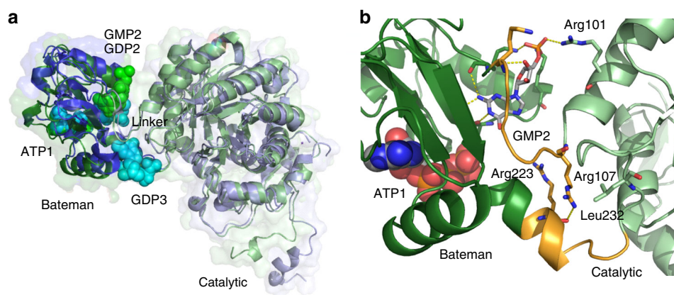
Fig. 6 Relative orientation of the catalytic and the regulatory domain. a Cartoon and surface representation of superposed monomers A from TbIMPDH-ATP1/GMP2 (green) and from AglIMPDH-ATP1/GDP2/GDP3 (blue, PDB 5TC3). Nucleotide atoms are shown as spheres. Both structures adopt an almost superimposable relative domain orientation. b Detailed view of the linker region (orange) between the Bateman (dark green) and the catalytic domains (light green) of TbIMPDH-ATP1/GMP2. The flipped conformation of GMP enables a direct interaction with residue Arg101 in the catalytic domain. Further stabilization is provided by an interaction of Arg107 and Arg223. ATP atoms are shown as spheres, while GMP and the GMP-binding residues as well as interface stabilizing residues are represented as sticks. Key interactions are shown as yellow dashes.
