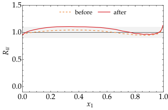
(a) \bar{u} momentum sum rule
