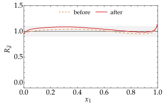
(b) \bar{d} momentum sum rule
