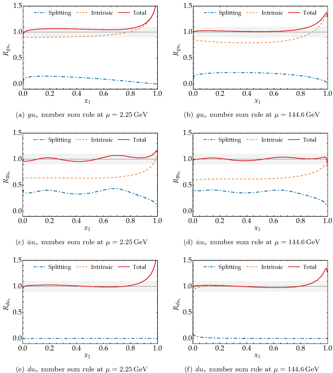
Figure 14: Comparison of number sum rule ratios for the final model at low and high scales. The contribution of the matching term is small and not shown.
