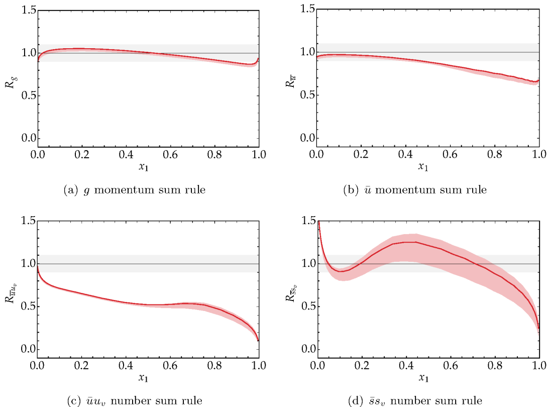
Figure 16: As figure 15, but for the initial DPD model described in section 3.
