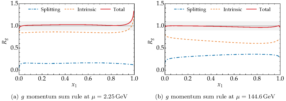
Figure 13: Comparison of the gluon momentum sum rule ratio for the final iteration of our model at two different scales. The contribution of the matching term is small and not shown.
