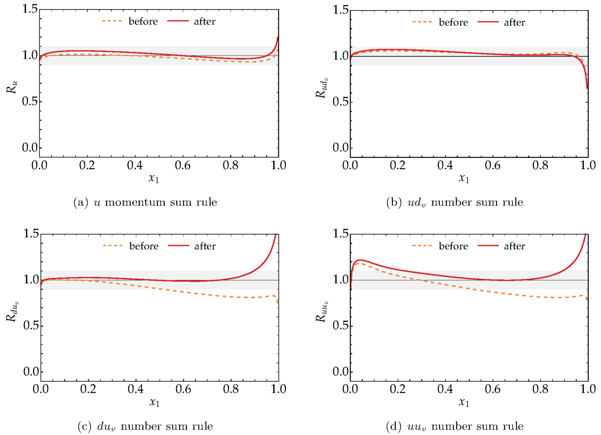
Figure 7: Sum rule ratios in the first and second interactions of the model, which respectively correspond to the powers (23) and (25) in the phase space factor.
