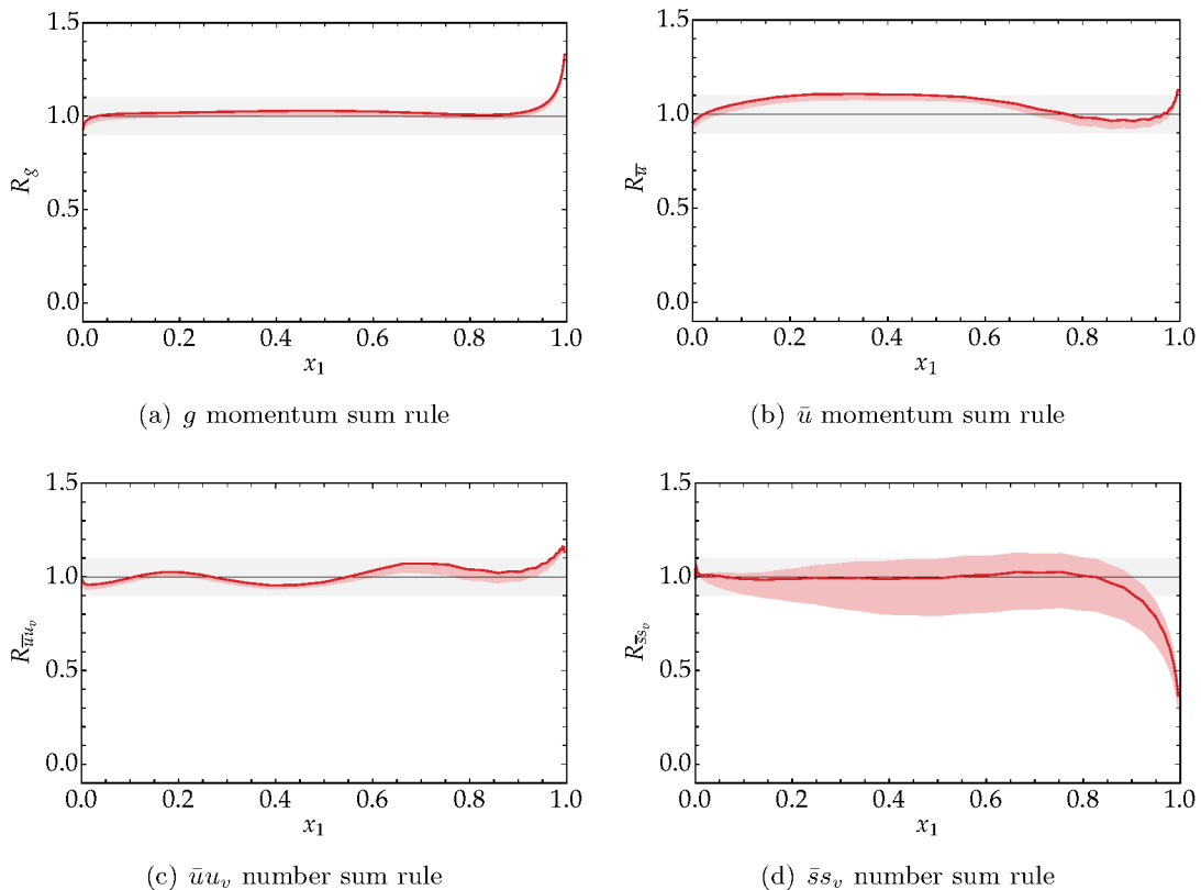
Figure 15: Cutoff scale dependence of sum rule ratios, evaluated at \mu = \mu_{\min} for the final iteration of our model. The solid curve is for \nu = \mu , and the band corresponds to a variation of \nu between \mu/2 and 2\mu .
