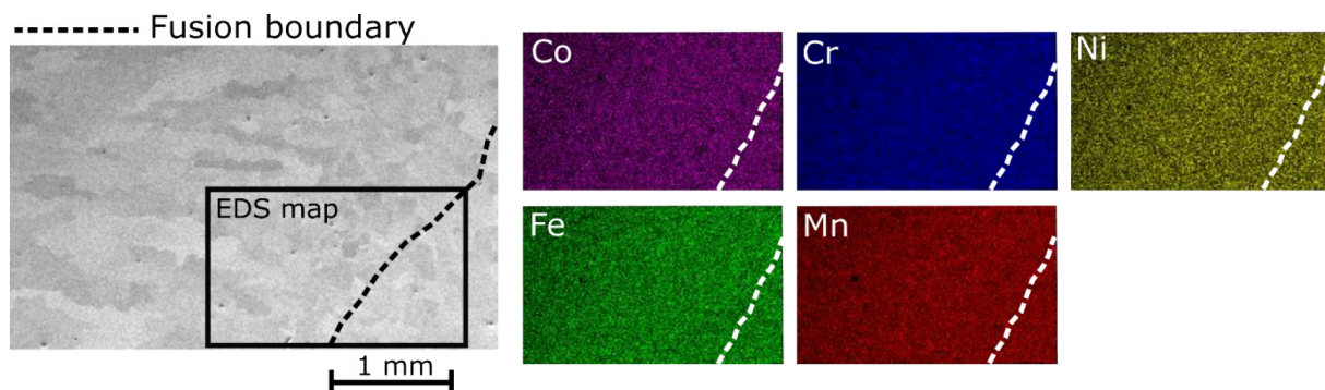
Fig. 4. EDS mapping across the fusion zone and heat affected zone.
