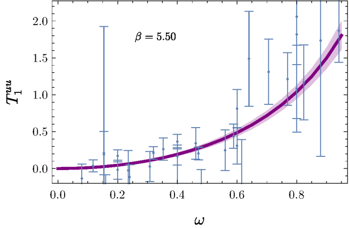
Figure 1: Compton amplitude extracted as a function of \omega = 2p \cdot q/Q^2 for five different Q^2 values (2.7...6.9 GeV 2 ). The curve shows a combined fit, as described in the text, including the leading-order perturbative QCD evolution (at a factorisation scale \mu^2 = 4\text{ GeV}^2 ).
