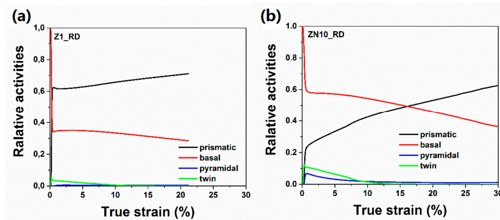
Figure 12. The relative deformation mode activities as a function of the strain: (a) Z1 along RD; (b) ZN10 along RD.
