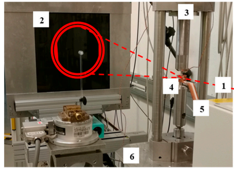
Figure 1. Beamline setup for texture measurement at HEMS P07B. Incoming hard X-ray and diffracted beam is marked with red line and circles.
