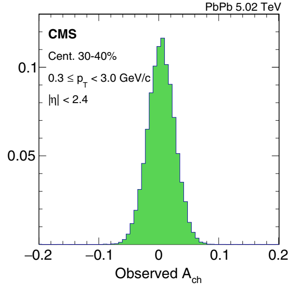
FIG. 1. The event-by-event probability distribution observed in the charge asymmetry, A_{\text{ch}} , for \text{PbPb} collisions at \sqrt{s_{\text{NN}}} = 5.02 TeV within the 30–40% centrality range. The particles are selected between 0.3 and 3.0 GeV/ c and having pseudorapidity |\eta| < 2.4 .
