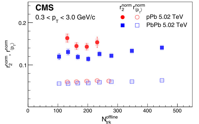
FIG. 4. The linear slope parameters r^{norm} for v_2 (filled symbols) and \langle p_T \rangle (open symbols) as functions of event multiplicity in p Pb and PbPb collisions at \sqrt{s_{NN}} = 5.02 TeV. Statistical and systematic uncertainties are indicated by the error bars and shaded regions, respectively.
