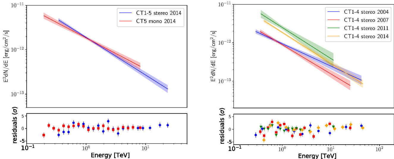
Fig. 2: Spectral energy distribution of gamma rays from PSR B1259–63/LS 2883. Left : Results obtained from the observation campaign in 2014, with two different instrument configurations: CT5 mono and CT1–5 stereo, shown in red and blue, respectively. Right : Results from observation campaigns in 2004, 2007, 2011 and 2014 in CT1–4 stereo mode. Spectral energy bins are defined such that flux points have a statistical significance above 2\sigma in all cases. The highest-energy flux point of the 2014 spectrum is significant at the 1.5\sigma level only. Upper panels show the best power-law fit to the data, with coloured bands indicating the 1\sigma statistical uncertainties on these fits. Lower panels provide the residuals of actual data to the best spectral fit. See main text for details.
