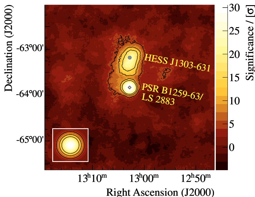
Fig. 1: Significance map of the region around PSR B1259–63/LS 2883 (white cross) obtained from the analysis of the 2014 data set in CT1–5 stereo mode. The pulsar wind nebula HESS J1303–631 (best-fit ellipse centre (Aharonian et al. 2005) indicated by a grey dot) is also detected to the north of PSR B1259–63/LS 2883. The bins in the map are correlated within a circle of radius 0.14^\circ . Significance contours are shown at the 5, 10, and 15\sigma levels. Some artefacts in the map are visible, occasionally exceeding the 5\sigma level, and are discussed in the text (see Sect. 4.1). In the inset, the point-spread function of the analysis is shown together with the respective contour lines.
