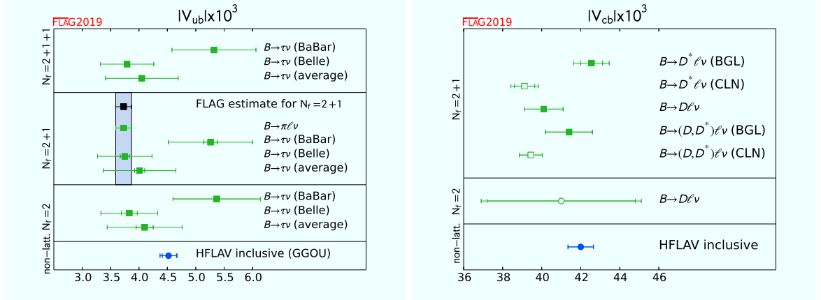
Figure 33: Left: Summary of |V_{ub}| determined using: i) the B -meson leptonic decay branching fraction, B(B^- \rightarrow \tau^- \bar{\nu}) , measured at the Belle and BaBar experiments, and our averages for f_B from lattice QCD; and ii) the various measurements of the B \rightarrow \pi \ell \nu decay rates by Belle and BaBar, and our averages for lattice determinations of the relevant vector form factor f_+(q^2) . Right: Same for determinations of |V_{cb}| using semileptonic decays. The HFLAV inclusive results are from Ref. [219, 653].
