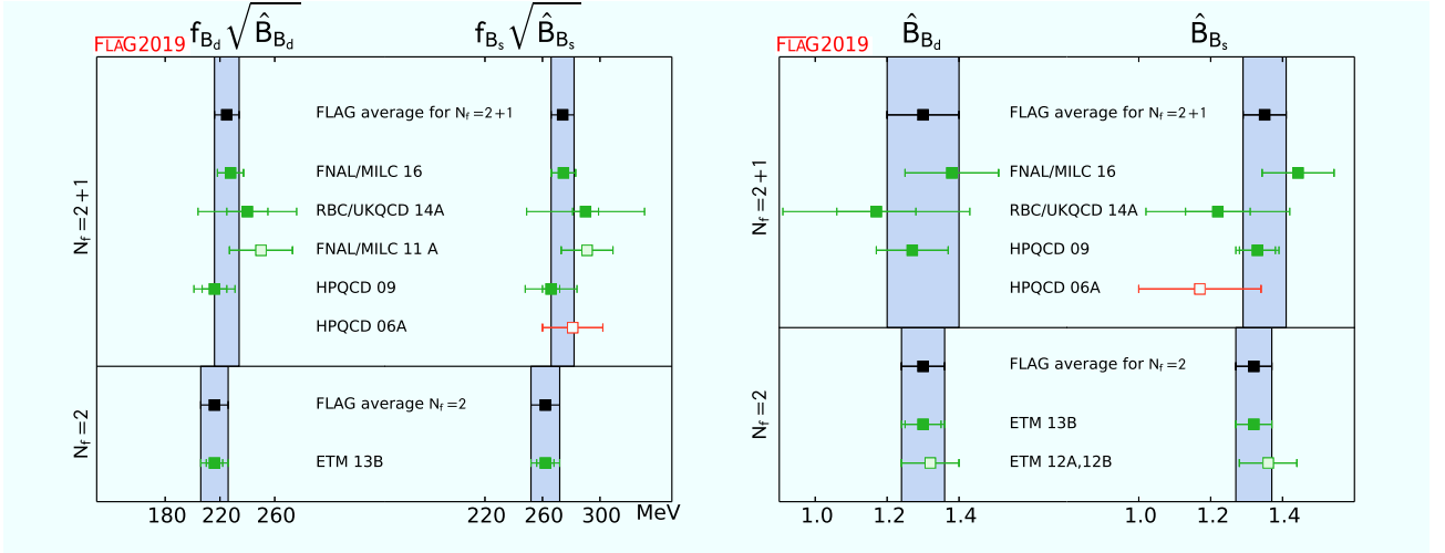
Figure 25: Neutral B - and B_s -meson mixing matrix elements and bag parameters [values in Tab. 36 and Eqs. (216), (219), (217), (220)].
