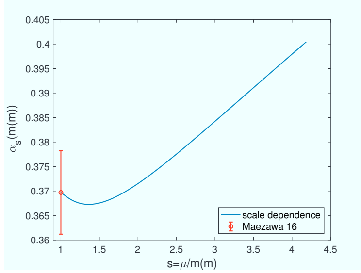
Figure 35: Renormalization-scale ( \mu ) dependence of \alpha(m_*) extracted from R_4 . We have evaluated this dependence for the case where the same renormalization scale is used for the quark mass and for \alpha_s .
