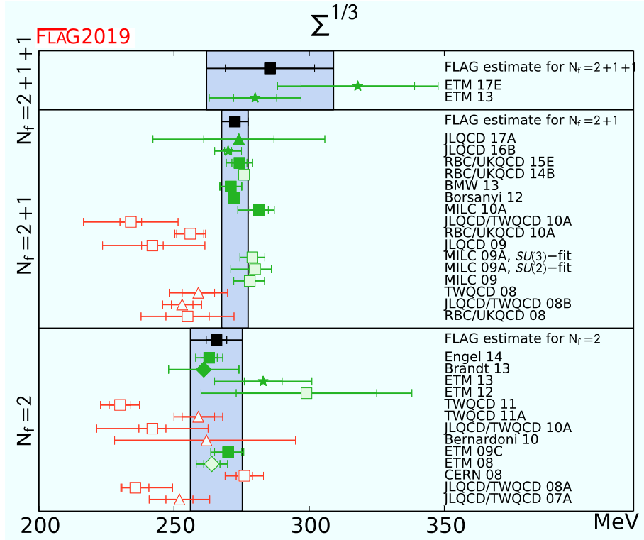
Figure 12: Cubic root of the SU(2) quark condensate \Sigma \equiv -\langle \bar{u}u \rangle|_{m_u, m_d \rightarrow 0} in the \overline{\text{MS}} -scheme, at the renormalization scale \mu = 2 \text{ GeV} . Green and red squares indicate determinations from correlators in the p -regime. Up triangles refer to extractions from the topological susceptibility, diamonds to determinations from the pion form factor, and star symbols refer to the spectral density method.
