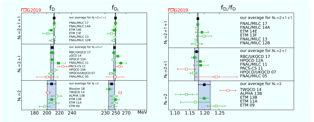
Figure 20: Decay constants of the D and D_s mesons [values in Tab. 30 and Eqs. (162-170)]. As usual, full green squares are used in the averaging procedure, pale green squares have been superseded by later determinations, while pale red squares do not satisfy the criteria. The black squares and grey bands indicate our averages.
