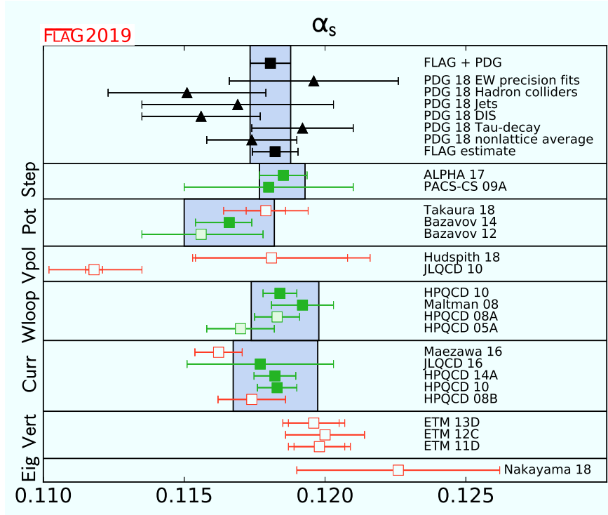
Figure 38: \alpha_{\overline{\text{MS}}}^{(5)}(M_Z) , the coupling constant in the \overline{\text{MS}} scheme at the Z mass. The PDG 18 entries give the outcome of their analysis from various phenomenological categories. The last PDG entry gives the outcome of their analysis excluding lattice results (see Sec. 9.10.4).
