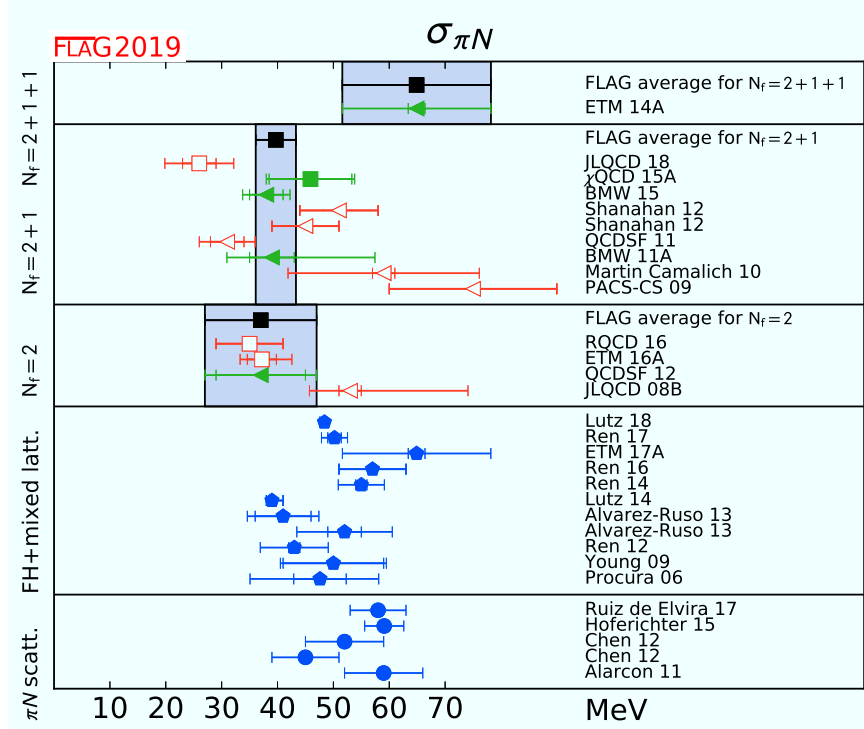
Figure 44: Lattice results and FLAG averages for the nucleon sigma term, \sigma_{\pi N} , for the N_f = 2, 2 + 1 , and 2 + 1 + 1 flavour calculations. Determinations via the direct approach are indicated by squares and the Feynman-Hellmann method by triangles. Results from calculations which analyse more than one lattice data set within the Feynman-Hellmann approach [452, 453, 945, 949–955] are shown for comparison (pentagons) along with those from recent analyses of \pi - N scattering [936–938, 956] (circles).
