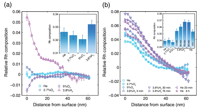
FIG. 3. Radial distributions of the relative Rh composition converted from compositional strain at 550 °C (a) and at 700 °C (b). The zeros of the relative Rh compositions were set to the mean values of the compositions in the core of 40 nm or larger from the surface. The displayed times in (b) are the elapsed times after the gas introductions. The insets exhibit the particle average compositions of Rh determined from the Bragg angles. These values are used to set the zeros in the vertical scale bars in Fig. 2. Error bars in the inset were estimated from the pixel size of the 2D detector.
