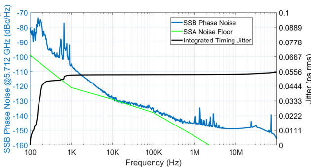
Figure 4: SSB Phase Noise for synthesized microwave from photodetection, Signal Source Analyzer (SSA) noise floor and absolute integrated timing jitter.
