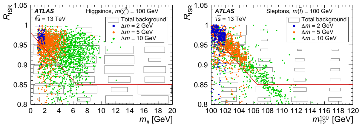
Figure 4: Distributions of R_{\text{ISR}} for the electroweakino (left) and slepton (right) high- E_{\text{T}}^{\text{miss}} SRs, after applying all signal selection criteria except those on R_{\text{ISR}} . The solid red line indicates the requirement applied in the signal region; events in the region below the red line are rejected. Representative benchmark signals for the higgsino (left) and slepton (right) simplified models are shown as circles. The gray rectangular boxes show the distribution of the total background expectations.
