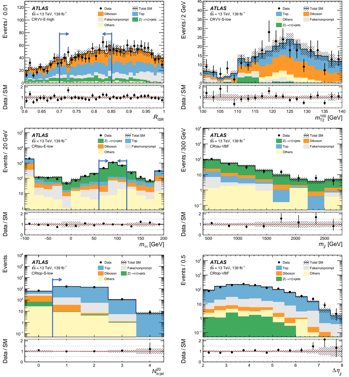
Figure 7: Examples of kinematic distributions after the background-only fit of the CRs showing the data as well as the expected background in the control regions CRVV-E-high (top left), CRVV-S-low (top right), CRtau-E-low (middle left), CRtau-VBF (middle right), CRtop-S-low (bottom left) and CRtop-VBF (bottom right). The full event selection of the corresponding regions is applied, except for distributions showing blue arrows, where the requirement on the variable being plotted is removed and indicated by the arrows in the distributions instead. The first (last) bin includes underflow (overflow). The uncertainty bands plotted include all statistical and systematic uncertainties.
