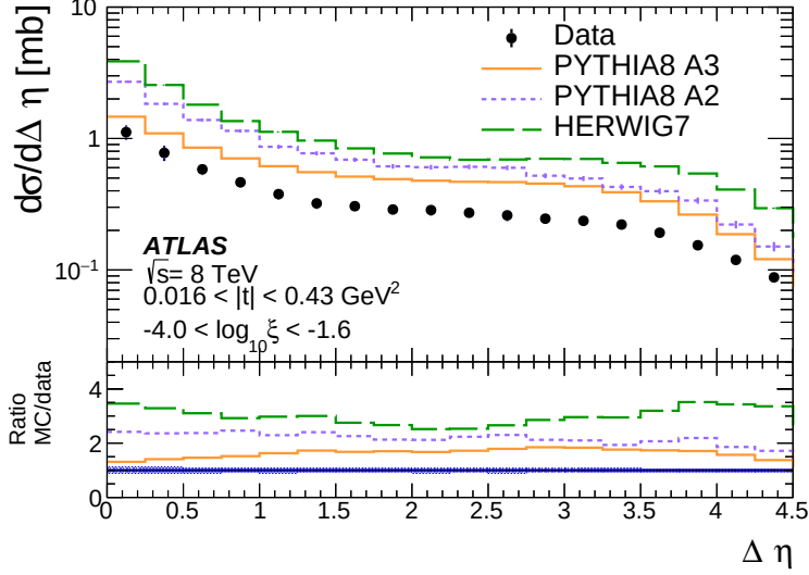
Figure 3: Hadron-level differential SD cross section as a function of \Delta\eta , comparing the measured data with PYTHIA8 and HERWIG7 predictions. The band around unity in the MC/data ratio shows the combination in quadrature of fractional statistical and systematic uncertainties.
