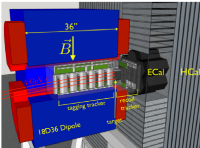
Figure 5: The LDMX experiment layout.
