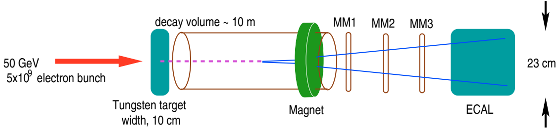
Figure 6: The AWAKE/NA64 conceptual layout.
