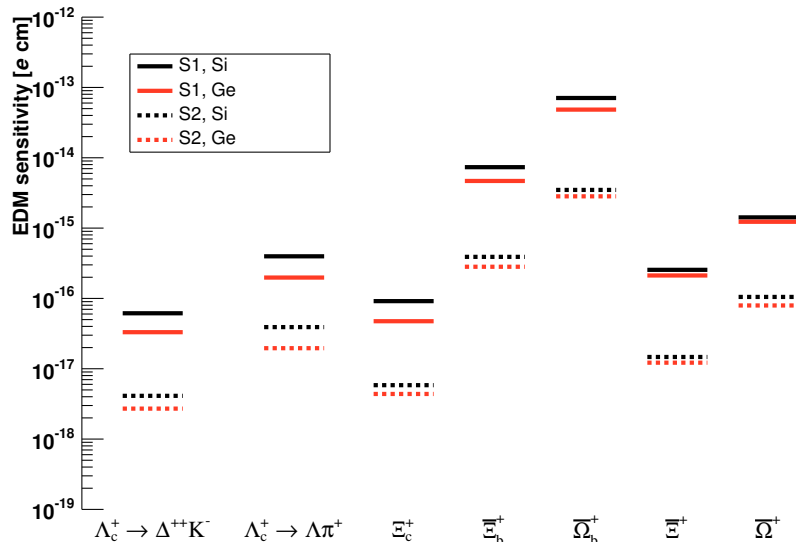
Figure 14: EDM sensitivities for different baryons in two different scenarios, scenario 1 (S1) corresponds to data collected at the LHCb interaction point in a first phase at low luminosity (about 2 \times 10^{14} pot); scenario 2 (S2) corresponds to data collected at a possible next-generation experiment at higher luminosity ( \sim 10^{17} ) and enhanced coverage. Figure revisited from Ref. [152].
