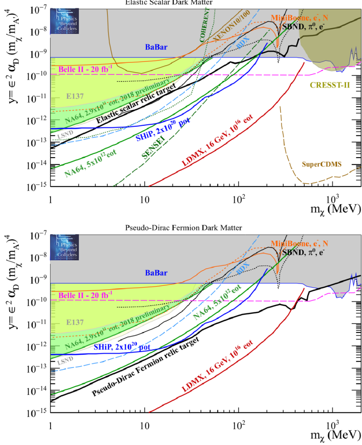
Figure 24: Dark Photon decaying to DM Elastic Scalar (top) or Pseudo-Dirac fermion (bottom) particle. Prospects for PBC projects on a timescale of 5 years ( \text{NA64}^{++} , green line) and 10-15 years (LDMX, red line and SHiP, blue line) are compared to the current bounds (solid areas) and future experimental landscape (other solid and dashed lines). In the limit computation we assume a dark coupling constant value \alpha_D = 0.1 and a ratio between the dark photon A' and LDM \chi masses m_{A'}/m_\chi = 3 .
