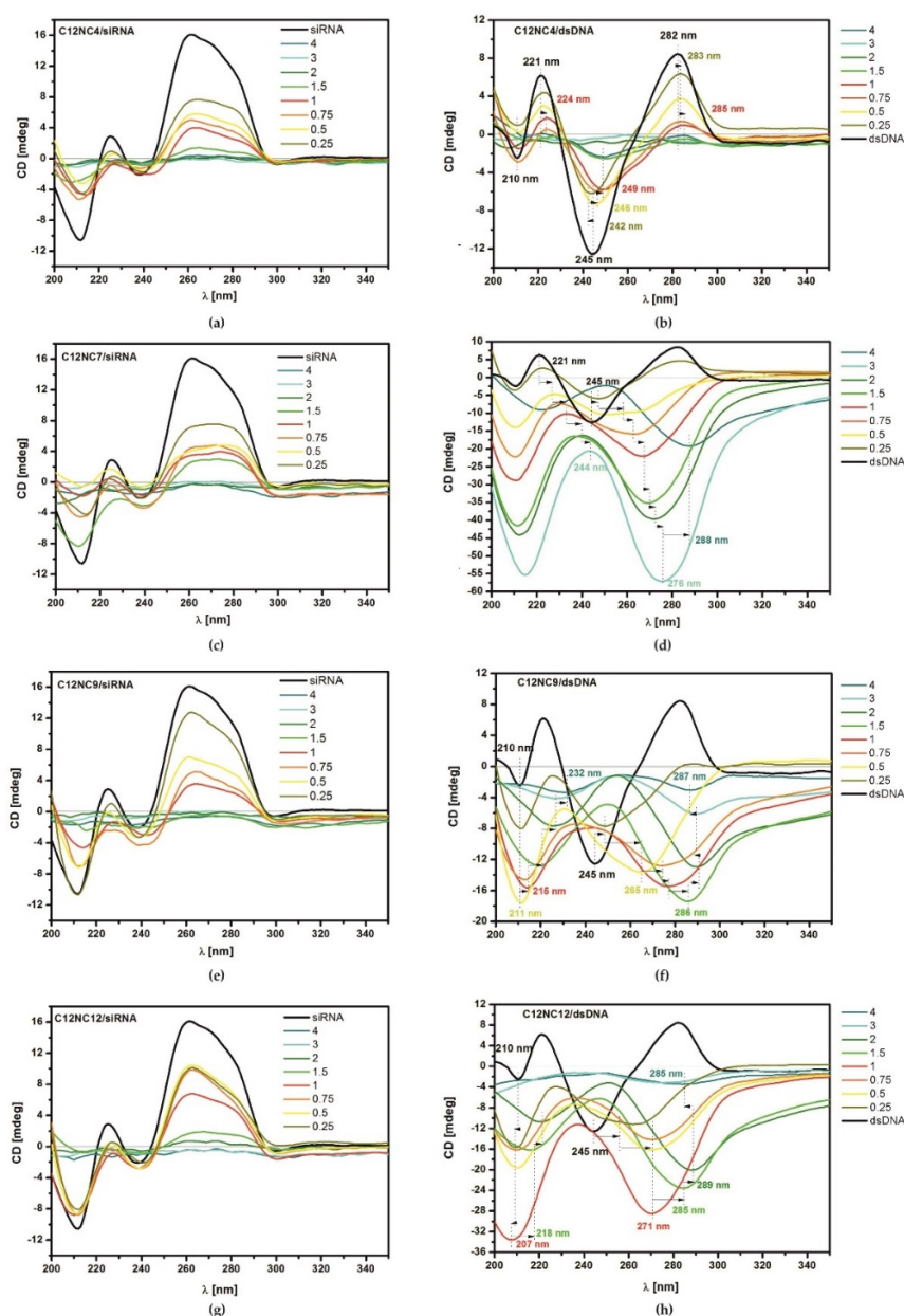
Figure 4. Circular dichroism results obtained for selected tested mixtures of C12NCn with siRNA (a,c,e,g) and dsDNA (b,d,f,h). The strongest signal which can be assigned to the Ψ-DNA phase was observed for C12NC7 for p/n = 3 (d).
