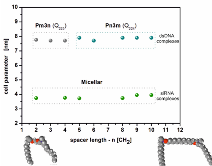
Figure 7. Spacing parameters for the cubic and micellar phase formed in the tested mixtures as a function of surfactants' spacer length. Molecular models – oxygen (red), nitrogen (blue), carbon (gray) and hydrogen (white).
