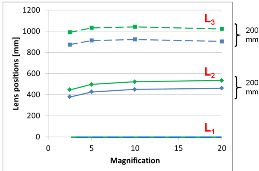
Figure 2. Simulated moving range of the telescope lenses for the required range of magnification.
