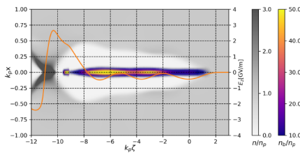
Figure 2: E_z Plotted for comb drive beam, TR ~ 8 (Architect)
