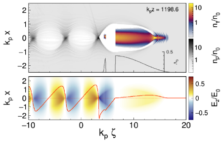
Figure 1: Snapshot shown for single drive beam, TR ~ 6 (HiPACE)
