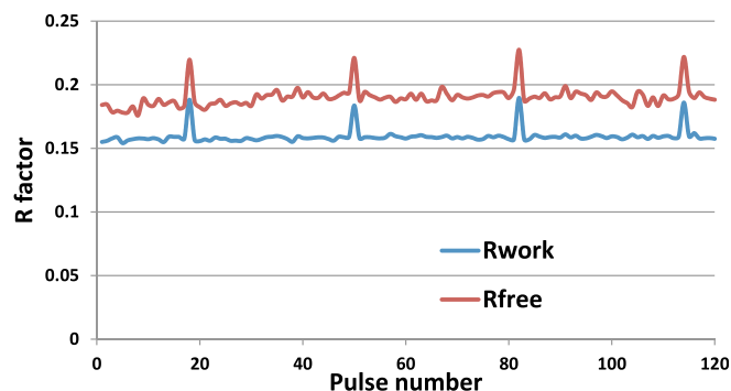
FIG. 6. R_{\text{free}} and R_{\text{work}} as a function of pulse number in the train.
