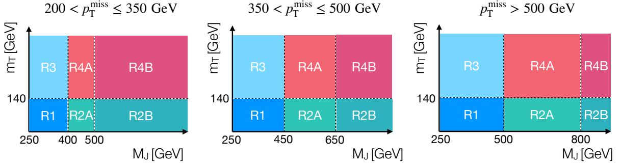
Figure 2: Analysis regions defined for each bin in p_T^{\text{miss}} . For the signal models considered here, the regions R1, R2A, R2B, and R3 are dominated by background, while R4A and R4B would have a significant signal contribution. In the combined fit performed to the event yields observed in these regions, signal contributions are allowed in the background-dominated regions. The R2A, R2B, R4A, and R4B regions are further divided into bins of N_{\text{jets}} and N_b , as discussed in the text.
