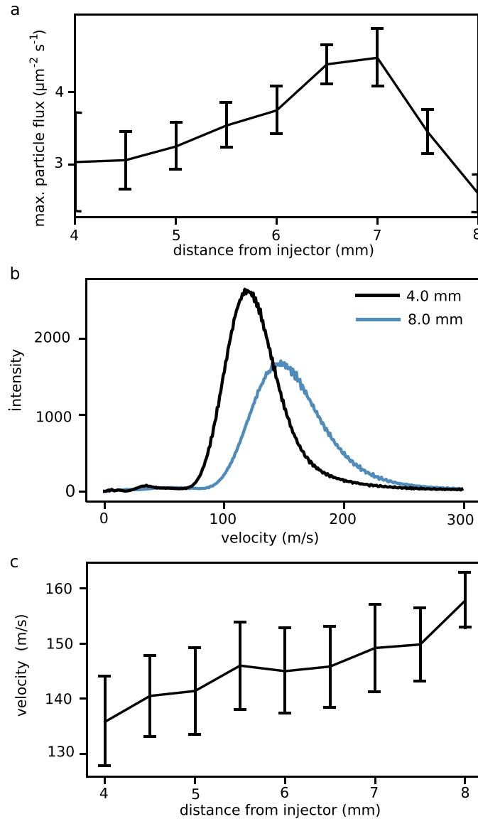
Fig. 3. (a) Maximum particle flux as a function of the distance from the ALS, vertical bars represent the standard errors. (b) Velocity distributions measured at distances of 4 mm (black) and 8 mm (blue) from the ALS. (c) Mean of the velocity distribution depending on the distance from the injector.
