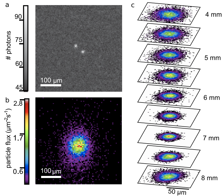
Fig. 2. (a) Raw image of a single camera frame containing two particles. (b) Transverse beam profile 6 mm below the injector tip, shown as a 2D histogram of the determined particle positions; the colorscale represents particle flux. (c) 3D beam profile shown as individual 2D histograms measured at different distances from the ALS exit. The colorscale is the same as in (b).
