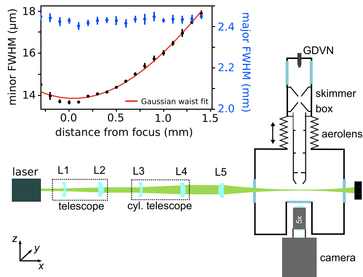
Fig. 1. Schematic of the light-sheet imaging setup for the characterization of nanoparticle beams emerging from an aerodynamic lens stack. The light sheet is generated using a spherical telescope, a cylindrical-lens telescope, and a spherical focusing lens to create an elliptical focus. The inset shows the measured values of the minor, z , and major, y , widths along the light beam and the corresponding Gaussian beam-waist fit to determine the Rayleigh length z_R = 1.5 mm. Light is detected with a microscope and camera setup along the y direction.
