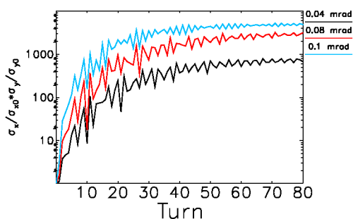
Figure 5: Normalized transverse beam size as a function of the number of turns for different values of kicks in both planes (1000 particles, \varepsilon_x = 17.4 pm rad, \varepsilon_y = 4 pm rad).
