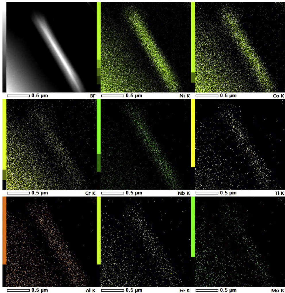
Fig. 7. STEM-HAADF image and EDS compositional maps of the elements identified in the sample VDM 780-a.
