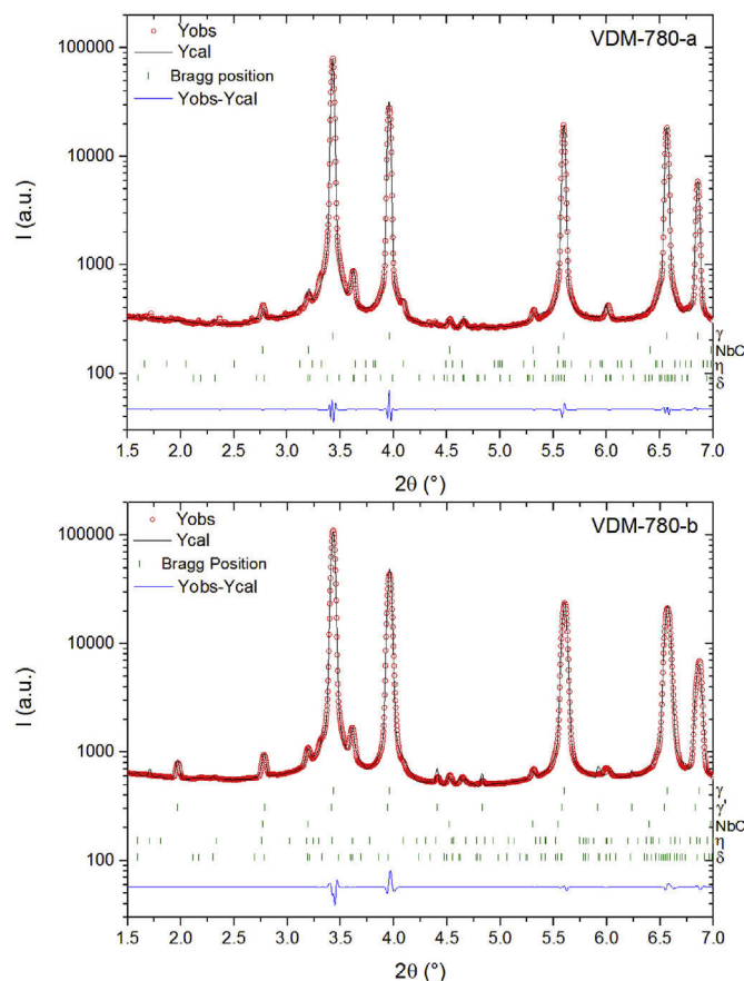
Fig. 2. The Rietveld refinement pattern (red circles: observed data and black line: calculated data) and difference plot (blue line) of the synchrotron data for the superalloy VDM 780-a and 780-b. The markers indicate the Bragg peak positions of the \gamma matrix, \gamma' phase, NbC, and the \eta and \delta high-temperature phases (from top to bottom). (For interpretation of the references to color in this figure legend, the reader is referred to the Web version of this article.)
