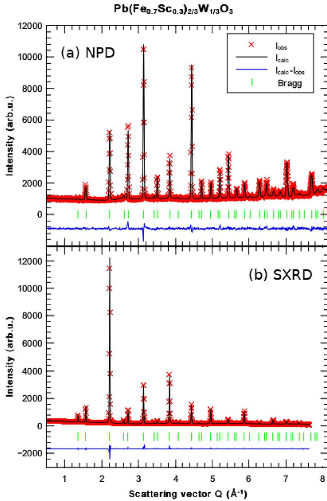
Fig. 9. Results of joint NPD + SXRPD refinements for the quenched \text{Pb}(\text{Fe}_{1-x}\text{Sc}_x)_{2/3}\text{W}_{1/3}\text{O}_3 sample with x = 0.3 ; T = 295 K (NPD: R_B : 4.40, R_p : 2.94, R_{wp} : 3.77; SXRPD: R_B : 3.73, R_p : 2.76, R_{wp} : 5.10).
