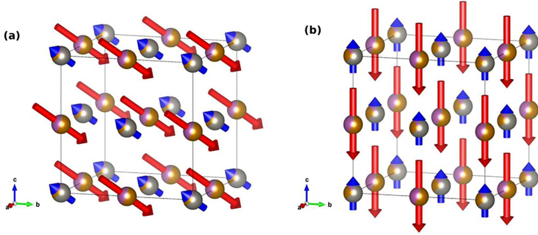
Fig. 12. Ferrimagnetic magnetic structure determined from the NPD data: (a) rhombohedral model ( R\bar{3}m' ) and (b) tetragonal model ( I4/mmm' ); drawn using VESTA [62].
