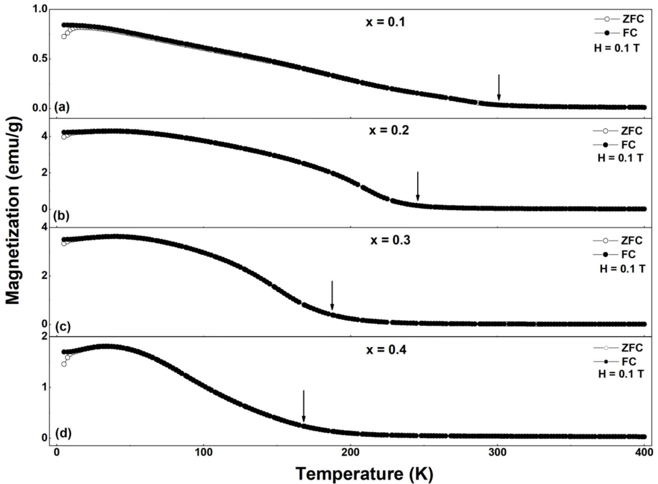
Fig. 6. ZFC/FC magnetization curves of the quenched \text{Pb}(\text{Fe}_{1-x}\text{Sc}_x)_{2/3}\text{W}_{1/3}\text{O}_3 samples ( 0.1 \leq x \leq 0.4 ); H = 1 \text{ kOe} . Arrows indicate the onset of magnetic ordering of the materials.
