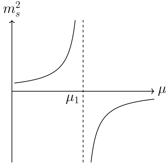
Figure 1: Schematic picture of the RG running of the scalaron mass squared m_s^2 .
