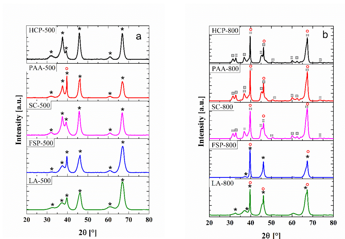
Figure 1: XRD patterns of a) calcined (500) and b) aged (800) samples with: * indicating diffraction peaks of \gamma\text{-Al}_2\text{O}_3 , ° of metallic Pt and □ of \theta\text{-Al}_2\text{O}_3 .
