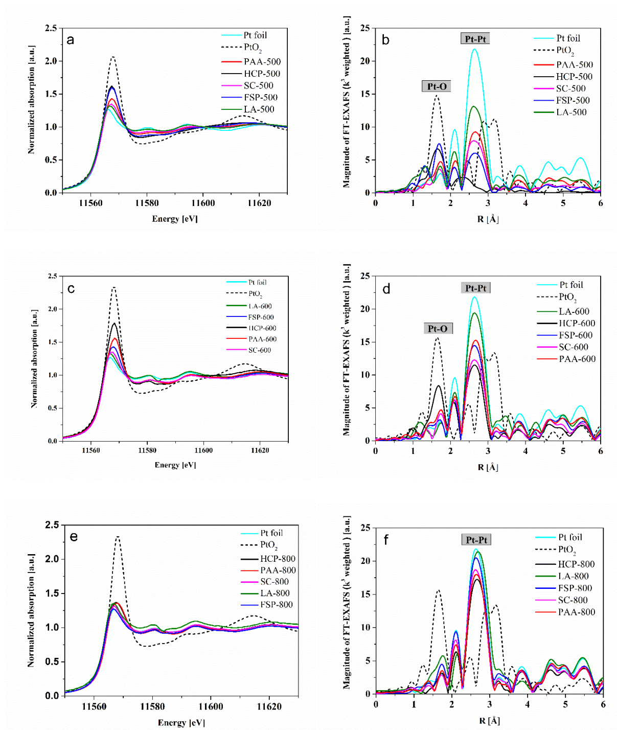
Figure 2: Pt \text{L}_3 XANES spectra of Pt/ \text{Al}_2\text{O}_3 a) calcined catalysts and after hydrothermal aging at c) 600 °C and e) 800 °C, including the reference samples, and b), d), f) the corresponding k^3 -weighted FT-EXAFS spectra.
