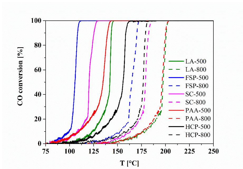
Figure 6: CO oxidation light-off of 3 rd cycle over differently prepared calcined (solid lines) and aged at 800 °C (dashed lines) Pt/Al 2 O 3 catalysts. Gas mixture: 500 ml/min of 1000 ppm CO, 10 % O 2 , N 2 with heating rate 5 °C min -1 , measured between 50-350 °C.
