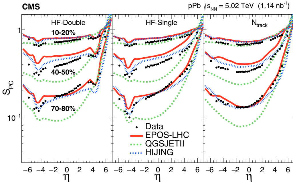
FIG. 5. Ratio of peripheral to central E_T production, S_{\text{PC}} , as a function of \eta for three centrality ranges for HF-double (left), HF-single (middle), and N_{\text{track}} (right) for data, and for the EPOS-LHC, QGSJET II, and HIJING event generators. The systematic uncertainties are dominant and are of comparable size to the data points.
