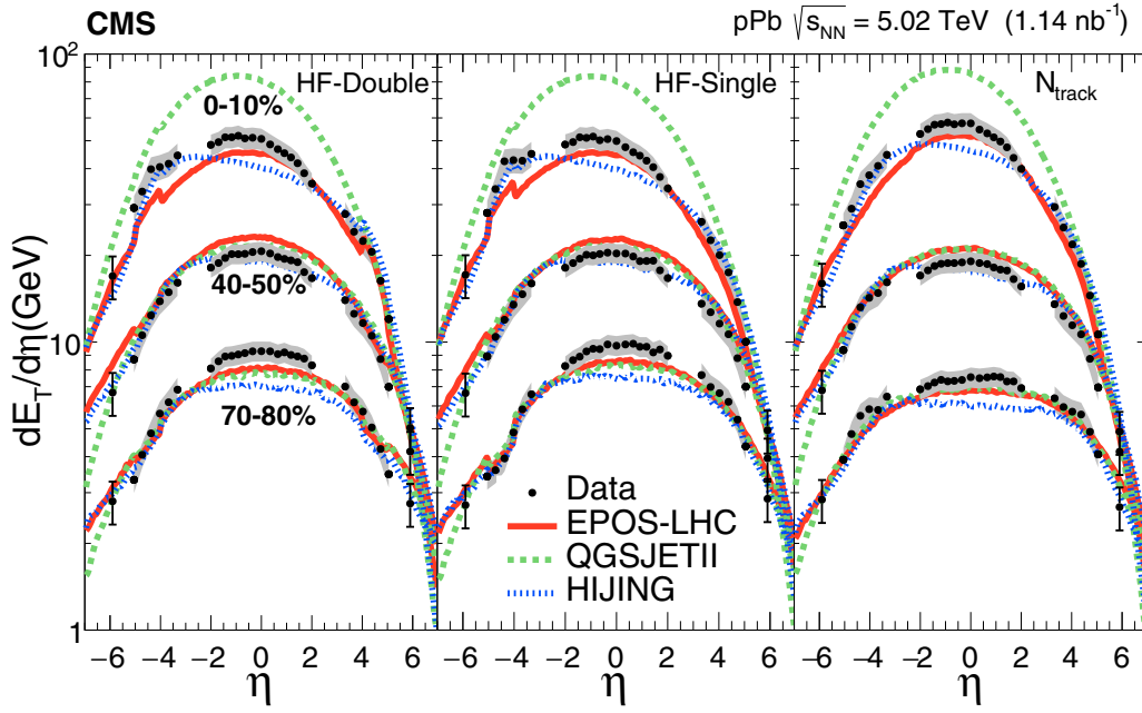
FIG. 3. Transverse energy density versus \eta and centrality from 5.02 TeV p Pb collisions for the HF-double (left), HF-single (center), and N_{\text{track}} (right) centrality definitions for data and for predictions from the EPOS-LHC, QGSJET II, and HIJING event generators, for 0–10% (upper), 40–50% (middle), and 70–80% (lower) central collisions. The uncertainties are dominated by the systematic components, which are largely correlated point-to-point in the central region and in HF and which are shown by gray bands there.
