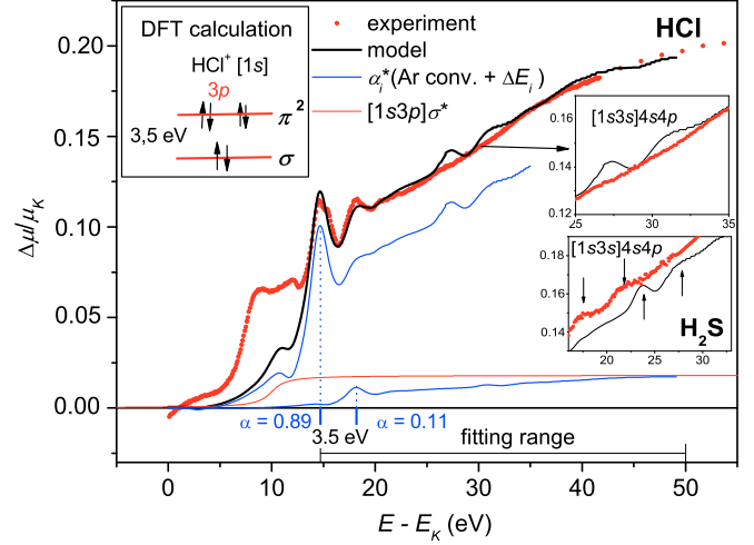
FIG. 5. Coexcitation spectrum of HCl. Experiment (red dots), the model of higher-energy part—quasiatomic coexcitations (black) and its components: the edge (red line), the shifted coexcitation spectra of Ar (blue line). The unmodeled low-energy part of the coexcitation spectrum corresponds to resonances involving the molecular orbitals. Insets: valence levels (left), the 3s coexcitation intervals of HCl and H 2 S (right).
