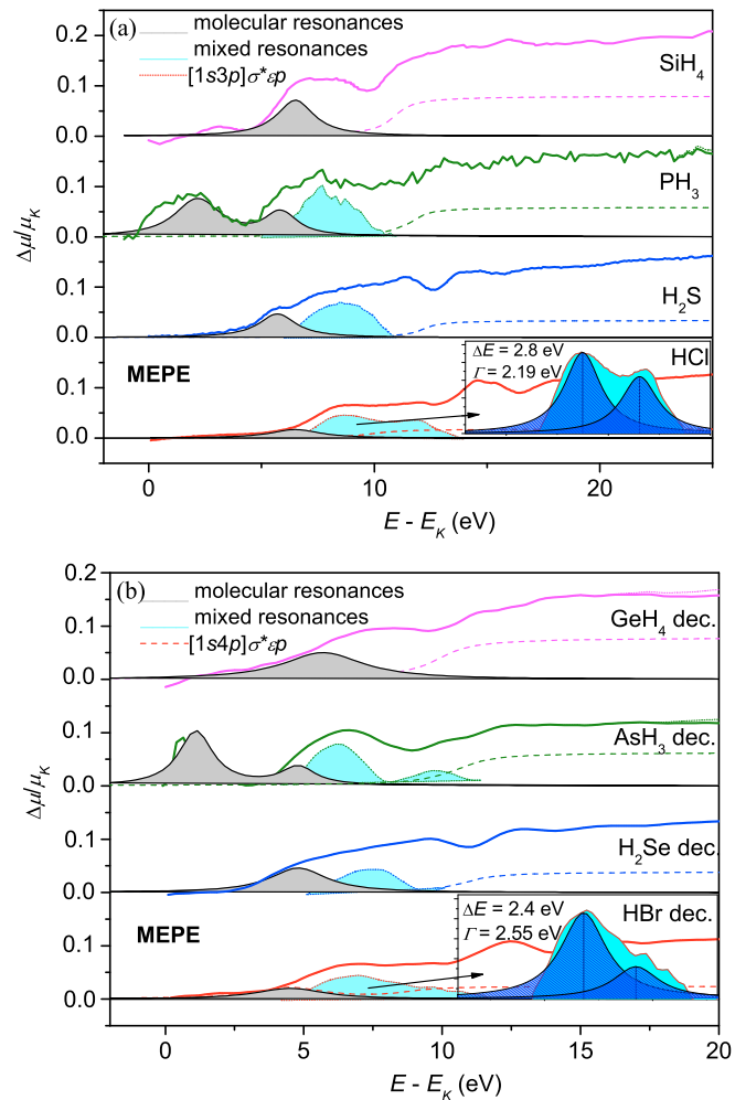
FIG. 8. Modeling the lower part of the MEPE spectrum (solid curve) for the 3p (a) and the deconvolved 4p series (b) includes resonant transitions into the [1sn(p, s)]\sigma^*\epsilon(p, s) final states (gray area) and shake-up into the [1sn(p, s)]\sigma^*\epsilon(p, s) final states (area under the dashed line). The residual (turquoise area) is attributed to the mixed-resonant channels. In the transparent insets, the model of mixed resonances in \text{HCl} and \text{HBr} , described in the text, is shown.
