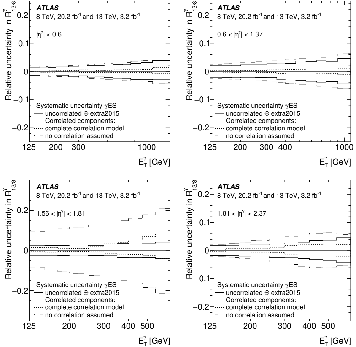
Figure 2. Relative systematic uncertainty in R_{13/8}^\gamma as a function of E_T^\gamma for different \eta^\gamma regions due to the \gamma ES correlated components (dashed lines). For comparison, the results of considering the components as uncorrelated are also shown (dotted lines) to illustrate the reduction in the size of the systematic uncertainty when the proper treatment is applied. The relative uncertainty due to the uncorrelated components of the photon energy scale and the components specific to 2015 is also shown (solid lines).
