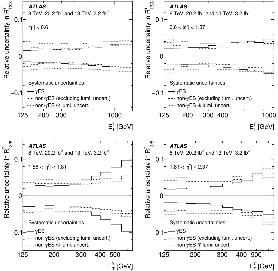
Figure 3. Relative systematic uncertainty in R_{13/8}^\gamma as a function of E_T^\gamma for different \eta^\gamma regions due to different sources: \gamma ES uncertainties (solid lines), non- \gamma ES uncertainties excluding the luminosity uncertainty (dashed lines) and non- \gamma ES and luminosity uncertainties added in quadrature (dotted lines).
