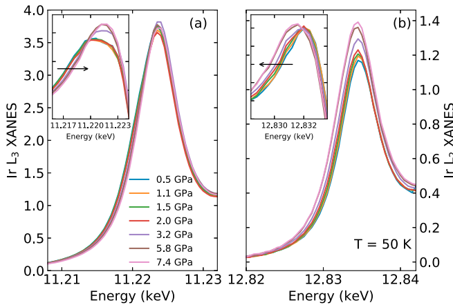
FIG. 6. (a) and (b) Ir L_{2,3} XANES data at T = 50\text{ K} for selected pressures. The insets show the first derivative of the XANES spectra and reveal the opposite energy shift behavior of the leading absorption edge as a function of pressure for each absorption edge.
