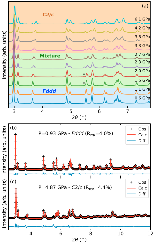
FIG. 8. (a) Angle dispersive x-ray powder diffraction of \beta - \text{Li}_2\text{IrO}_3 as a function of pressure at T = 11 K. At \sim 1.5 GPa, a new weak peak around 2\theta = 5.45^\circ appears (marked by *), followed by more new peaks after \sim 2 GPa. Refinements of the diffraction patterns indicate a mixture of phases between 1.5–3.3 GPa. After 3.3 GPa, the XRD patterns could be refined within the pure C2/c space group. (b) and (c) LeBail refinements using pure Fddd and C2/c structures.
