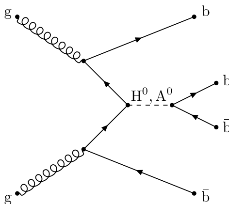
Figure 3.1: Feynman-Diagram showing the production and decay of a heavy Higgs boson.
