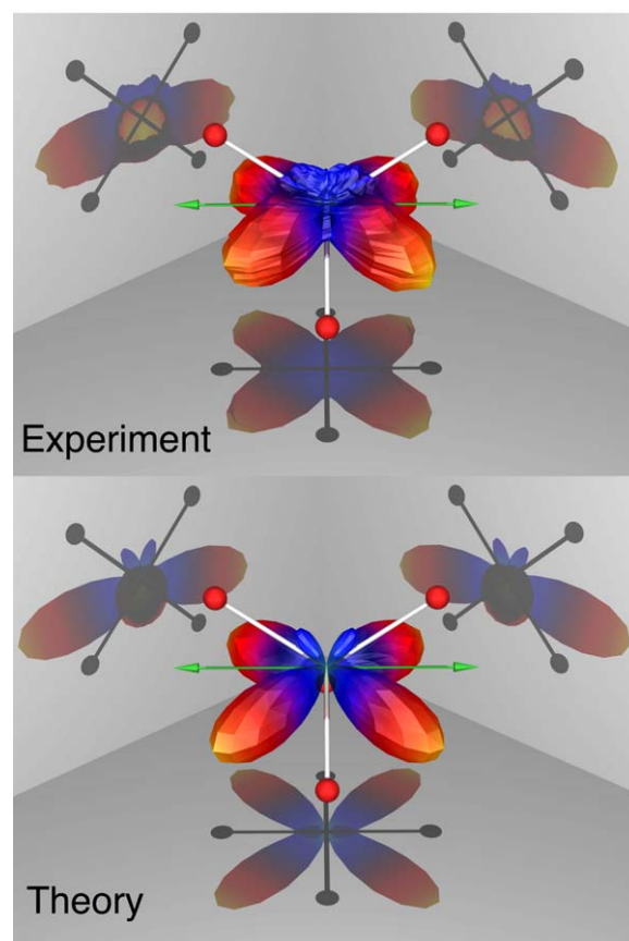
Figure 21. MFPAD for carbon K-shell photoionization of CF 4 with linearly polarized light from frozen-core Hartree–Fock theory and experiment where the photoelectron was measured in coincidence with two F + atoms produced after an Auger decay. Reproduced from [162]. © IOP Publishing Ltd. All rights reserved. The four red balls in the central images give the location of the F atoms and the double headed green arrow gives the direction of the polarization. The four-lobe MFPAD pattern indicates strong scattering from the F atoms.
