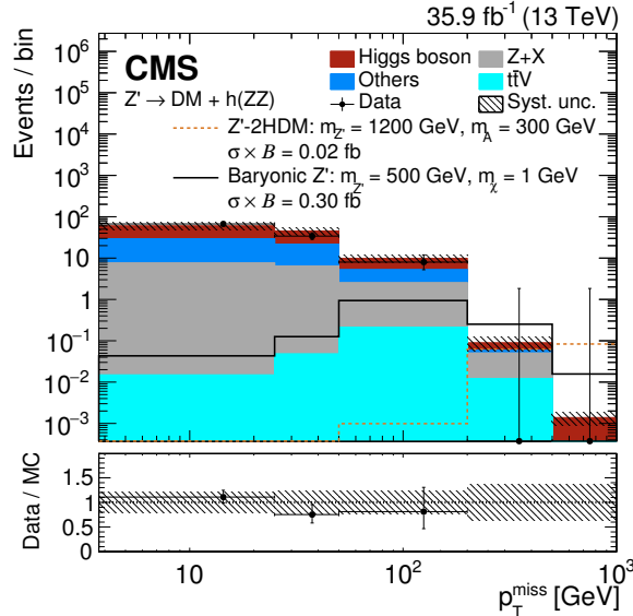
Figure 6: The p_T^{\text{miss}} distribution for the expected background and observed events in data in the h \rightarrow \text{ZZ} analysis. Two signal benchmarks, corresponding to the Z' -2HDM (dotted orange line, left) and baryonic Z' (solid black line, right) model are superimposed. The signal is normalized to the product of cross section and branching fraction, where \mathcal{B} represents the h \rightarrow \text{ZZ} branching fraction. The systematic uncertainties are shown by the hatched band. The ratios of the data and the sum of all the SM backgrounds are shown in the bottom panels.
