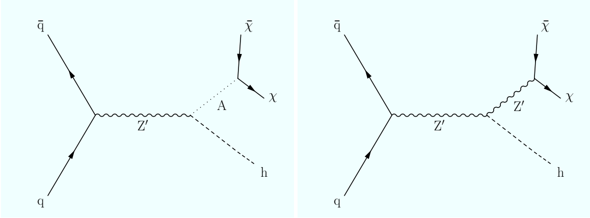
Figure 1: Representative Feynman diagrams for the two benchmark signal models considered in this paper: the Z' -2HDM (left) and the baryonic Z' model (right).
