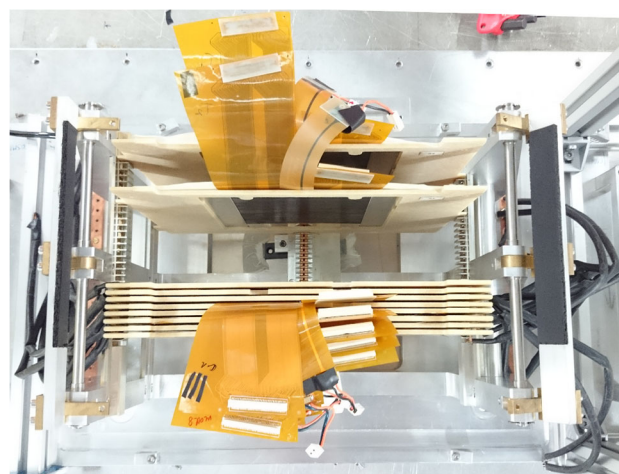
Fig. 6 Top view of the assembled calorimeter
