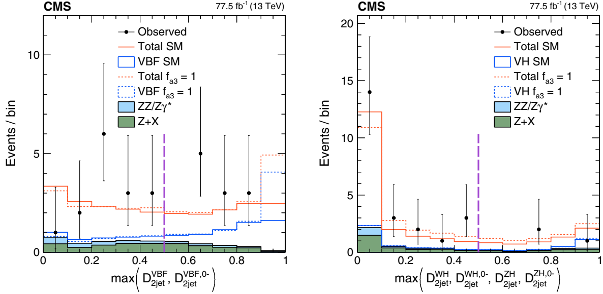
FIG. 2. The distributions of events for \max(\mathcal{D}_{2\text{jet}}^{\text{VBF}}, \mathcal{D}_{2\text{jet}}^{\text{VBF},0-}) (left) and \max(\mathcal{D}_{2\text{jet}}^{\text{WH}}, \mathcal{D}_{2\text{jet}}^{\text{WH},0-}, \mathcal{D}_{2\text{jet}}^{\text{ZH}}, \mathcal{D}_{2\text{jet}}^{\text{ZH},0-}) (right) in the on-shell region in the data from 2016 and 2017 from the analysis of the a_3 coupling for a pseudoscalar contribution. The requirement \mathcal{D}_{\text{bkg}} > 0.5 is applied in order to enhance the signal contribution over the background. The VBF signal under both the SM and pseudoscalar hypotheses is enhanced in the region above 0.5 for the former variable, and the WH and ZH signals are similarly enhanced in the region above 0.5 for the latter variable.
