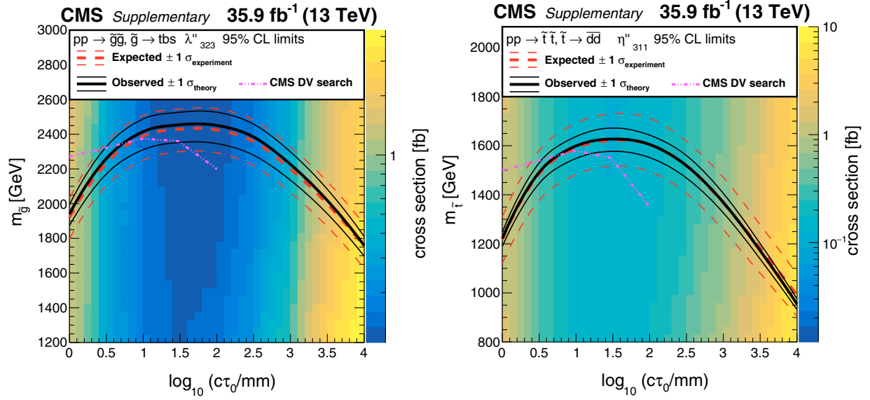
FIG. 8. Comparison with search for displaced vertices in multijet events at \sqrt{s} = 13 TeV with the CMS detector [36] (referred to as the CMS DV search) for \tilde{g} \rightarrow tbs (left) and \tilde{t} \rightarrow \bar{d}d (right) models. The CMS DV search looks for a pair of displaced vertices within the beam pipe. The observed limits obtained by the CMS DV search (purple curves) are overlaid with the limits obtained by the search presented in this paper in the mass-lifetime plane, and are good complements for proper decay length c\tau_0 < 10 mm in these two signal models.
