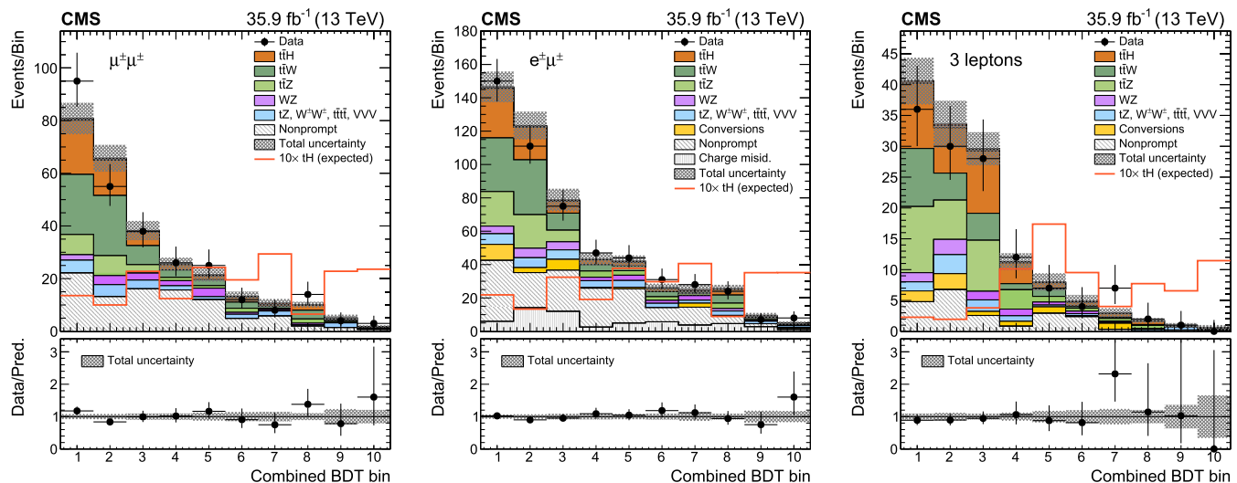
FIG. 6. Postfit categorized classifier outputs as used in the maximum likelihood fit for the \mu^\pm\mu^\pm channel (left), e^\pm\mu^\pm channel (center), and three-lepton channel (right), for 35.9 \text{ fb}^{-1} . In the box below each distribution, the ratio of the observed and predicted event yields is shown. The shape of the tH signal is indicated with ten times the SM.
