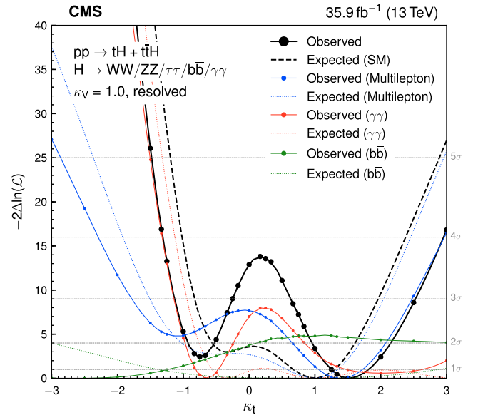
FIG. 13. Scan of -2\Delta\ln(\mathcal{L}) vs \kappa_t for the data (black line) and the individual channels (blue, red, and green), compared to Asimov data sets corresponding to the SM expectations (dashed lines).
