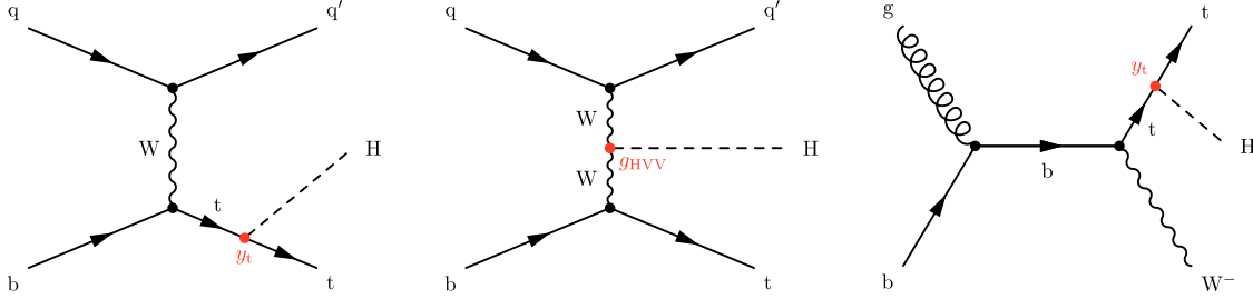
FIG. 1. Leading-order Feynman diagrams for the associated production of a single top quark and a Higgs boson in the t channel, where the Higgs boson couples to either the top quark (left) or the W boson (center), and one representative diagram of tHW production, where the Higgs boson couples to the top quark (right).
