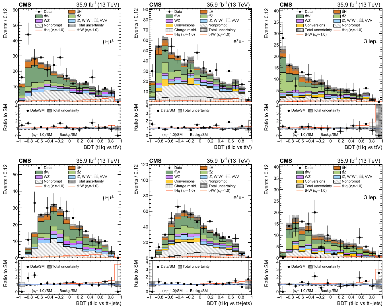
FIG. 5. Prefit classifier outputs, for the \mu^+\mu^+ channel (left), e^+\mu^+ channel (center), and three-lepton channel (right), for training against t\bar{t}V (top row) and against t\bar{t} + \text{jets} (bottom row). In the box below each distribution, the ratio of the observed and predicted event yields is shown. The shape of the two tH signals for \kappa_t = -1.0 is shown, normalized to their respective cross sections for \kappa_t = -1.0 , \kappa_t = 1.0 . The grey band represents the unconstrained (prefit) statistical and systematic uncertainties.
