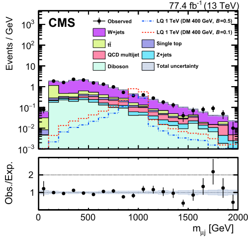
Fig. 3. The observed distribution of m_{lj} in comparison to the post-fit SM background predictions for the combined 2016 and 2017 data. “Post-fit” means that the constraints from the maximum likelihood fit are incorporated. The unstacked predictions for two signal models with m_{LQ} = 1000 GeV and m_{DM} = 400 GeV are also shown with B = 0.5 and the other with B = 0.1 . The difference is just an overall relative normalization of about 2 for the latter compared to the former. The ratio of the observed results to the total SM prediction is shown in the lower panel. The vertical error bars on the data points are statistical. The gray shows the total uncertainty in the background prediction, including both statistical and systematic terms.
