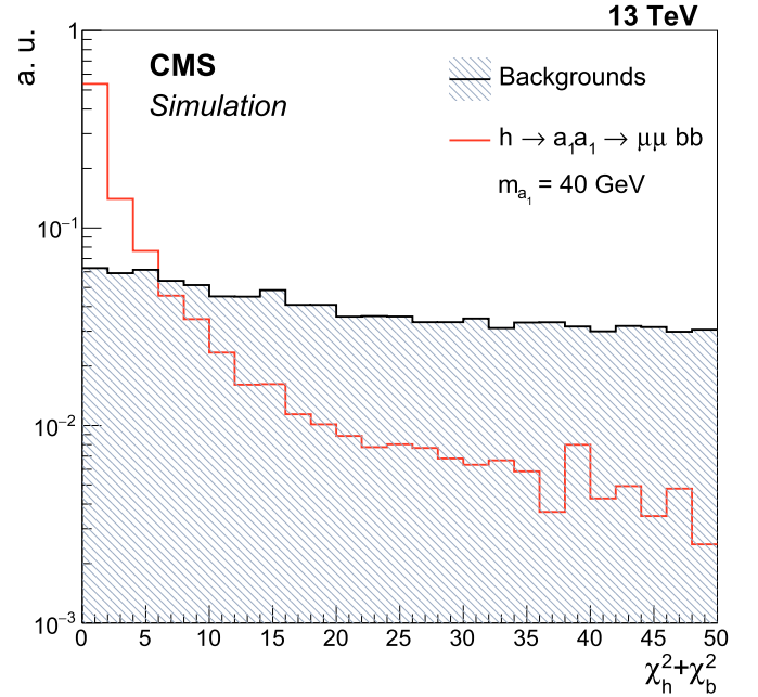
Fig. 1. The distribution of \chi^2 in simulated background processes and the signal process with m_{a_1} = 40 GeV. The samples are normalised to unity.
