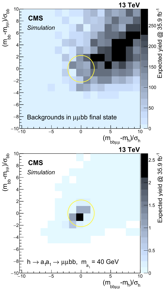
Fig. 2. The distribution of \chi_{bb} versus \chi_h as defined in Eq. (2) for (upper) simulated background processes and (lower) the signal process with m_{a_1} = 40 \text{ GeV} . The contours encircle the area with \chi^2 < 5 . The grey scale represents the expected yields at 35.9 \text{ fb}^{-1} .
