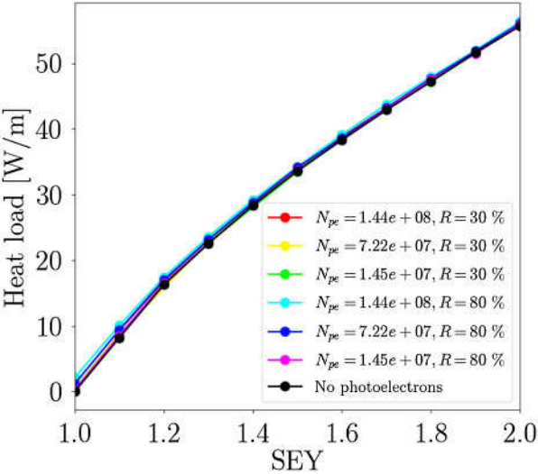
Fig. 2.34. Heat load as a function of SEY for arc dipoles for the case with no photoelectrons and for various values of photoelectrons and reflectivity.
