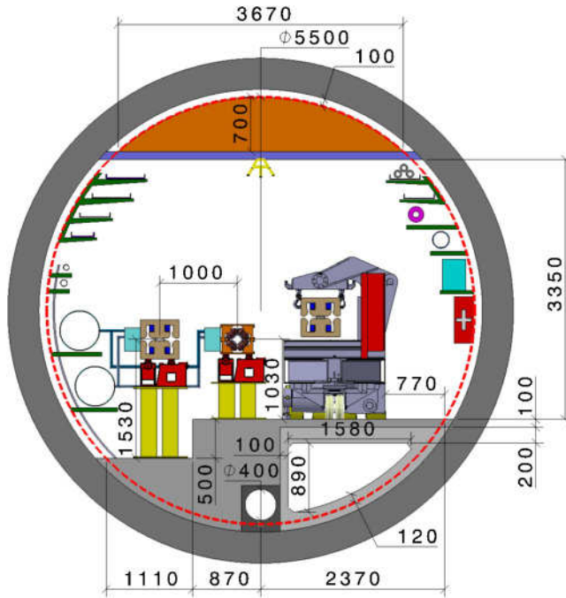
Fig. 2.4. Cross-section of the tunnel in the arc region. The dual-aperture magnets of the collider ring are located towards the outside of the ring tunnel (left), with the magnets of the booster more towards the inside of the ring tunnel (middle). A magnet installation vehicle travels along the transport passage.
