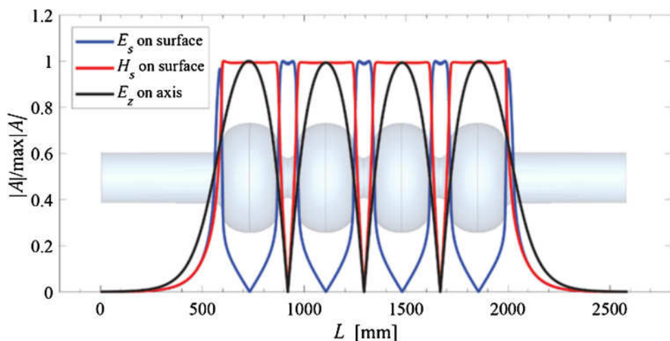
Fig. 3.17. Drawing of a four-cell Nb/Cu cavity at 400.79 MHz, proposed for the WW and ZH modes of operation, including field profiles.
