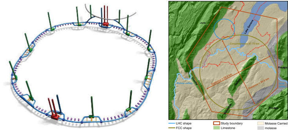
Fig. 5. Left: 3D, not-to-scale schematic of the underground structures. Right: study boundary (red polygon), showing the main topographical and geological structures, LHC (blue line) and FCC tunnel trace (brown line).
