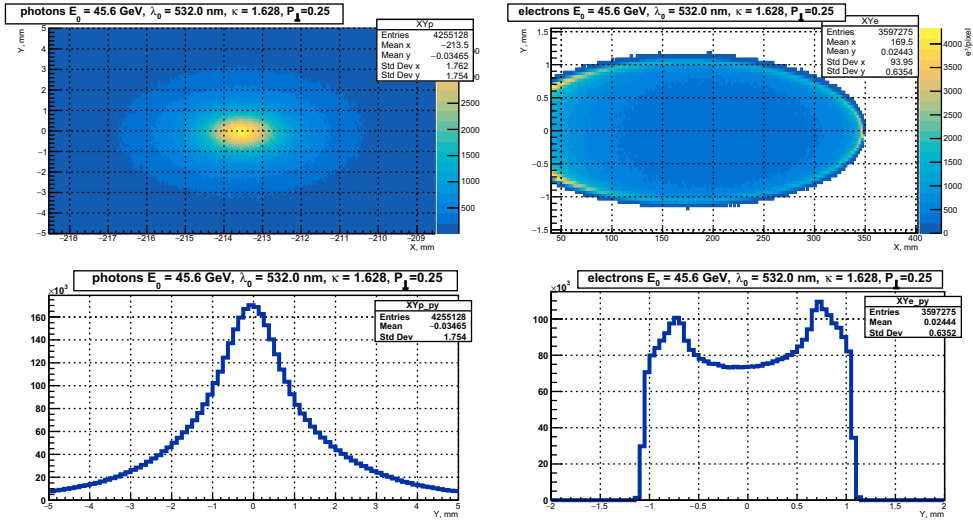
Fig. 3.29. MC results for P_{\perp} = \xi_{\chi}\xi_{\perp} = 0.25 and \phi_{\perp} = \pi/2 .
