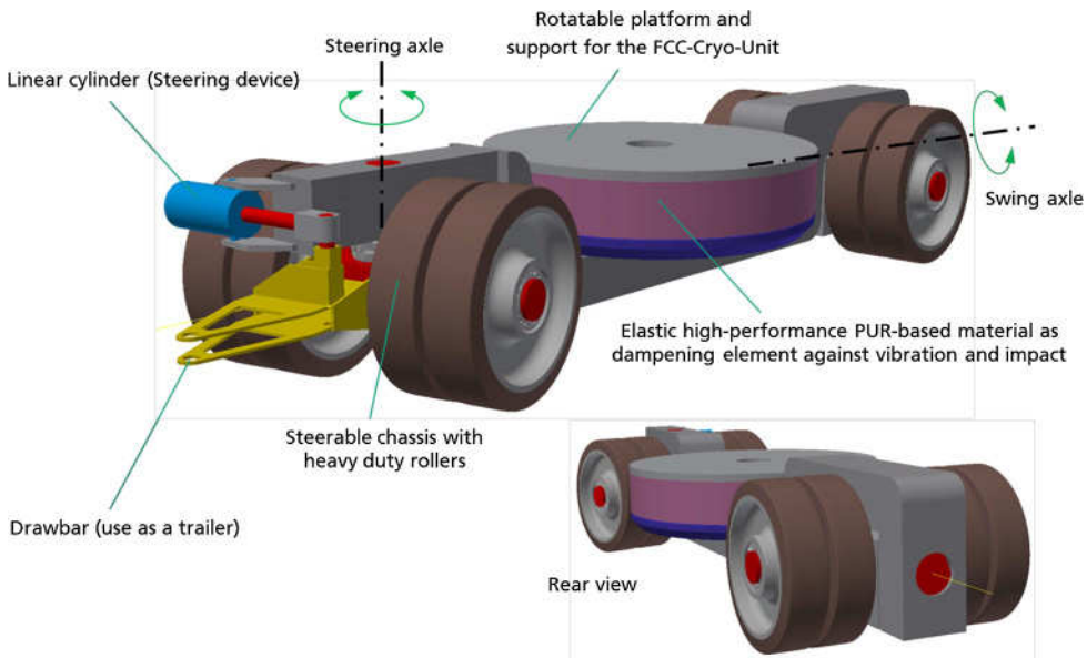
Fig. 5.16. A conceptual view of a trailer.
