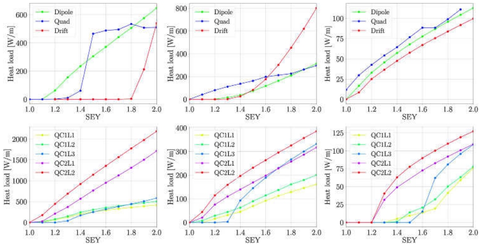
Fig. 2.33. Heat load as a function of SEY for arc components (top) and IR magnets (bottom) for 2.5 ns (left side), 5 ns (center) and 15 ns (right side) bunch spacings.
