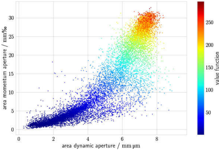
Fig. 2.14. Value function as a function of area of momentum aperture and area of dynamic aperture for all solutions of the PSO algorithm.
