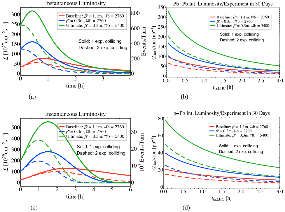
Fig. 2.12. Left: instantaneous luminosity evolution. Right: optimum average integrated luminosity as a function of the LHC turnaround time, assuming 100% efficiency and machine availability. In 2016 the LHC achieved a minimum turnaround time of 2.5 h [149]. With a faster cycling LHC (see Sect. 2.5) the theoretical optimum of the LHC turnaround for an ion cycle could be around 28 min, depending on the filling scheme. (a) Pb–Pb instantaneous luminosity. (b) Pb–Pb integrated luminosity. (c) p–Pb instantaneous luminosity. (d) p–Pb integrated luminosity.
