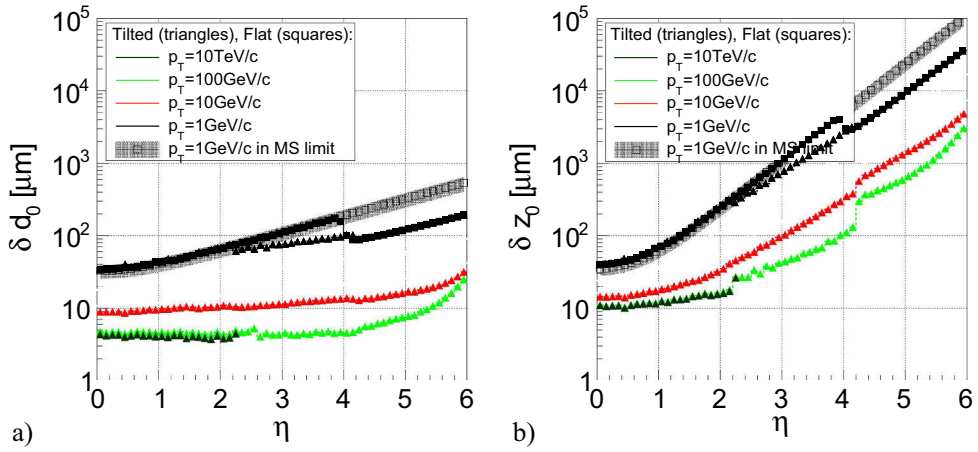
Fig. 7.13. (a) Transverse impact parameter resolution. (b) Longitudinal impact parameter resolution. The open symbols in both figures represent elementary formulae for high p_T and multiple scattering limits.
