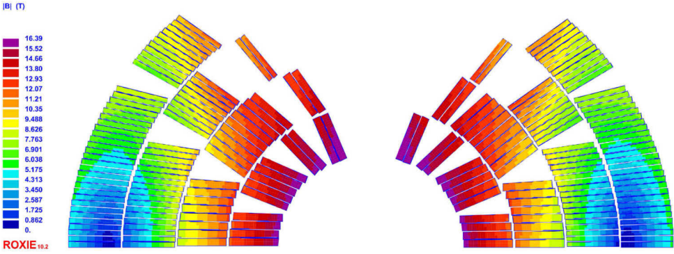
Fig. 3.3. Conductor distribution and field amplitude in the coil (half aperture).
