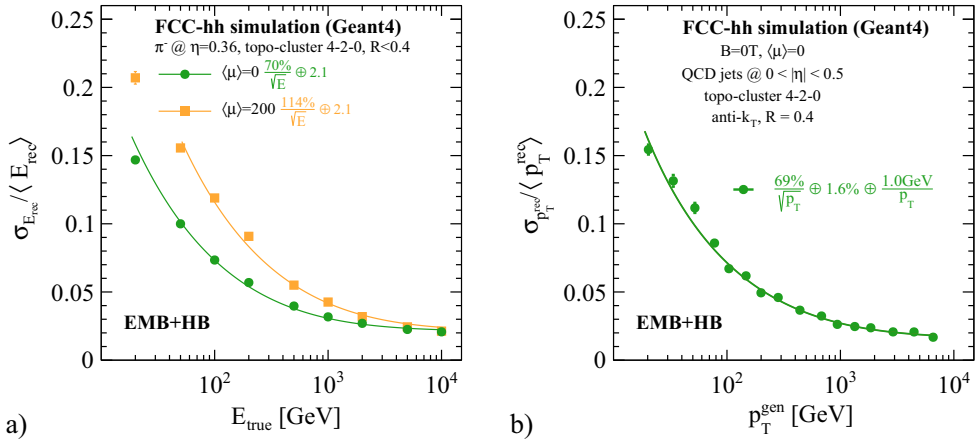
Fig. 7.19. (a) Single pion resolution using for barrel EMB + HB at \eta = 0.36 and B = 4\text{ T} with electronics noise only (green circles) and for a pile-up of \langle \mu \rangle = 200 (orange squares). Only clusters with \Delta R < 0.4 from the generated particle direction are included. (b) Momentum resolution for jets in the barrel EMB + HB at B = 0\text{ T} and without pile-up using the anti- k_T jet cone algorithm on top of the cluster reconstruction.
