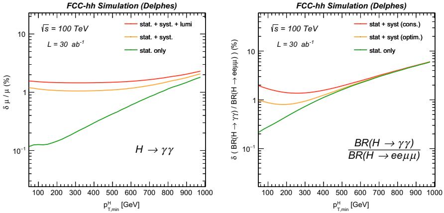
Fig. 1.2. Examples of projected precision for Higgs measurements with 30\text{ ab}^{-1} . Left: H \rightarrow \gamma\gamma production rate at large p_T . Right: ratio of H \rightarrow \gamma\gamma and H \rightarrow 2e2\mu rates. The results labelled as “cons” are obtained by doubling the default systematic uncertainties for \gamma , e and \mu efficiencies.
