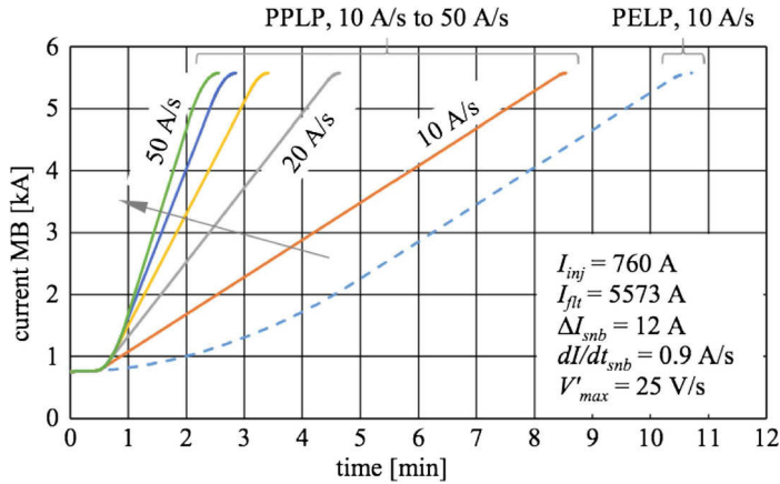
Fig. 6.6. 450 GeV–3.3 TeV LHC ramps, showing the gain from a PPLP ramp with different linear ramp rates between 10 and 50 A/s, compared to the present LHC PELP ramp (dashed).
