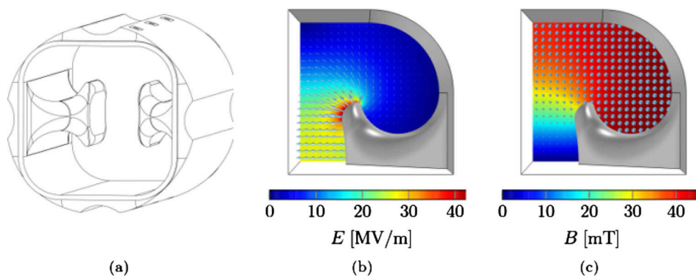
Fig. 3.16. (a) Design of the wide-open-waveguide crab cavity. The electric (b) and magnetic (c) fields of the fundamental mode are scaled to the nominal deflecting voltage of V_{\perp} = 3 MV.
