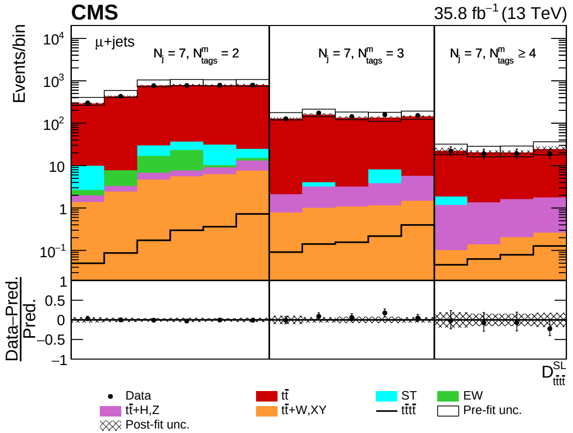
Figure 6: Post-fit D_{\text{t}\bar{\text{t}}\text{t}\bar{\text{t}}}^{\text{SL}} distribution in the single-muon channel for events satisfying baseline single-lepton selection and N_j = 7 , N_{\text{tags}}^m = 2, 3, \geq 4 . Non-uniform binning of the BDT discriminant was chosen to achieve approximately uniform distribution of the \text{t}\bar{\text{t}} background. Dots represent data. Vertical error bars show the statistical uncertainties in data. The post-fit background predictions are shown as shaded histograms. Open boxes demonstrate the size of the pre-fit uncertainty in the total background and are centered around the pre-fit expectation value of the prediction. The hatched area shows the size of the post-fit uncertainty in the background prediction. The signal histogram template is shown as a solid line. The lower panel shows the relative difference of the observed number of events over the post-fit background prediction.
