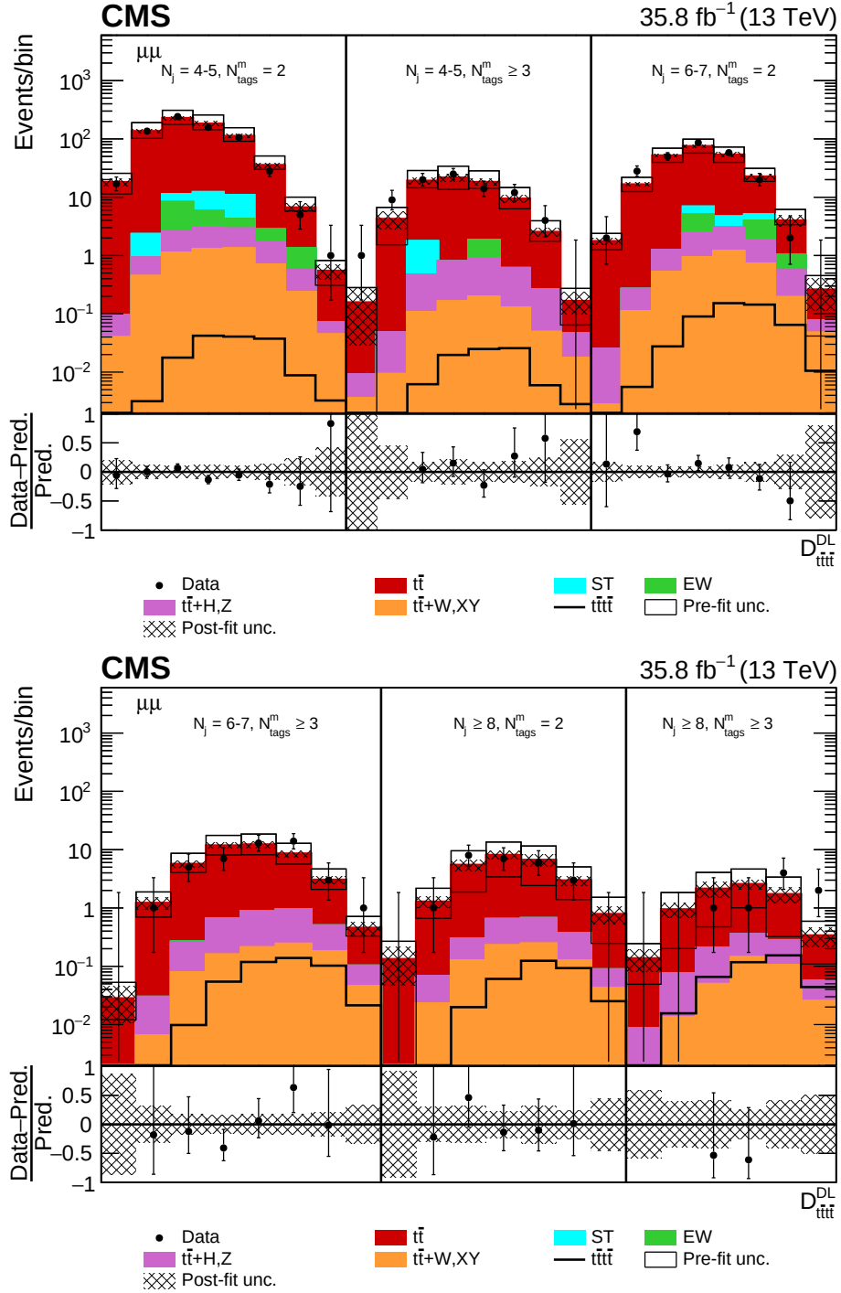
Figure 10: Post-fit D_{tt\bar{t}\bar{t}}^{DL} distributions in the \mu^+\mu^- channel for events satisfying baseline opposite-sign dilepton selection and (upper row) N_j = 4-5, N_{\text{tags}}^m = 2, \geq 3, N_j = 6-7, N_{\text{tags}}^m = 2 and (lower row) N_j = 6-7, N_{\text{tags}}^m \geq 3, N_j \geq 8, N_{\text{tags}}^m = 2, \geq 3 . Dots represent data. Vertical error bars show the statistical uncertainties in data. The post-fit background predictions are shown as shaded histograms. Open boxes demonstrate the size of the pre-fit uncertainty in the total background and are centered around the pre-fit expectation value of the prediction. The hatched area shows the size of the post-fit uncertainty in the background prediction. The signal histogram template is shown as a solid line. The lower panel shows the relative difference of the observed number of events over the post-fit background prediction.
