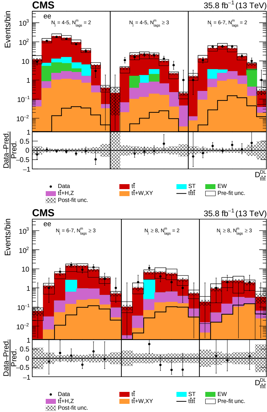
Figure 12: Post-fit D_{t\bar{t}t\bar{t}}^{DL} distributions in the e^+e^- channel for events satisfying baseline opposite-sign dilepton selection and (upper row) N_j = 4-5, N_{\text{tags}}^m = 2, \geq 3, N_j = 6-7, N_{\text{tags}}^m = 2 and (lower row) N_j = 6-7, N_{\text{tags}}^m \geq 3, N_j \geq 8, N_{\text{tags}}^m = 2, \geq 3 . Dots represent data. Vertical error bars show the statistical uncertainties in data. The post-fit background predictions are shown as shaded histograms. Open boxes demonstrate the size of the pre-fit uncertainty in the total background and are centered around the pre-fit expectation value of the prediction. The hatched area shows the size of the post-fit uncertainty in the background prediction. The signal histogram template is shown as a solid line. The lower panel shows the relative difference of the observed number of events over the post-fit background prediction.
