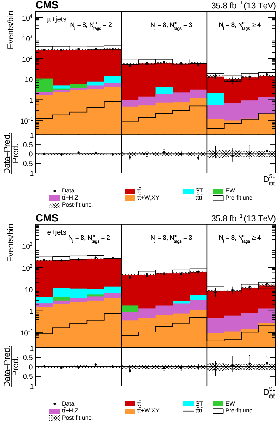
Figure 7: Post-fit D_{\text{tt}}^{\text{SL}} distribution in the (upper row) single-muon and (lower row) single-electron channels for events satisfying baseline single-lepton selection and N_j = 8, N_{\text{tags}}^m = 2, 3, \geq 4 . Non-uniform binning of the BDT discriminant was chosen to achieve approximately uniform distribution of the t\bar{t} background. Dots represent data. Vertical error bars show the statistical uncertainties in data. The post-fit background predictions are shown as shaded histograms. Open boxes demonstrate the size of the pre-fit uncertainty in the total background and are centered around the pre-fit expectation value of the prediction. The hatched area shows the size of the post-fit uncertainty in the background prediction. The signal histogram template is shown as a solid line. The lower panel shows the relative difference of the observed number of events over the post-fit background prediction.
