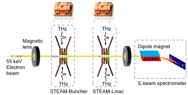
Fig. 1. Schematic illustration of the experimental setup. 55 keV electron bunches are generated by a DC electron gun. The UV pulses are produced from a part of the Yb:YLF laser pulses by two SHG stages and directed onto a gold photocathode generating photoelectrons, which are further accelerated to 55 keV by the DC electric field between the photocathode and anode plate. This Yb:YLF laser also drives four synchronized optical-rectification stages, each generating single-cycle terahertz pulses. The STEAM-buncher is driven by two counterpropagating terahertz beams with energy \sim 2 \times 50 nJ for electron compression. The STEAM-linac is driven by \sim 2 \times 15 \mu J terahertz radiation for electron acceleration.
