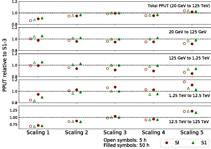
Figure 10: Relative PPUT values for different energy ranges for the layout with a hexagonal MST pattern (“S1”) and a layout with an MST pattern presenting four islands (“SI”), both for the southern site, relative to “S1-3”. Open and filled symbols correspond to observation times of 5 h and 50 h, respectively.
