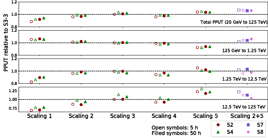
Figure 11: Relative PPUT values for different energy ranges for several CTA-South layout candidates, relative to “S3-3”. The resulting PPUT values obtained by combining the MST layout with moderate radial scaling (2) and the SST layout with strong scaling (5) are shown labelled as “scaling 2+5”.
