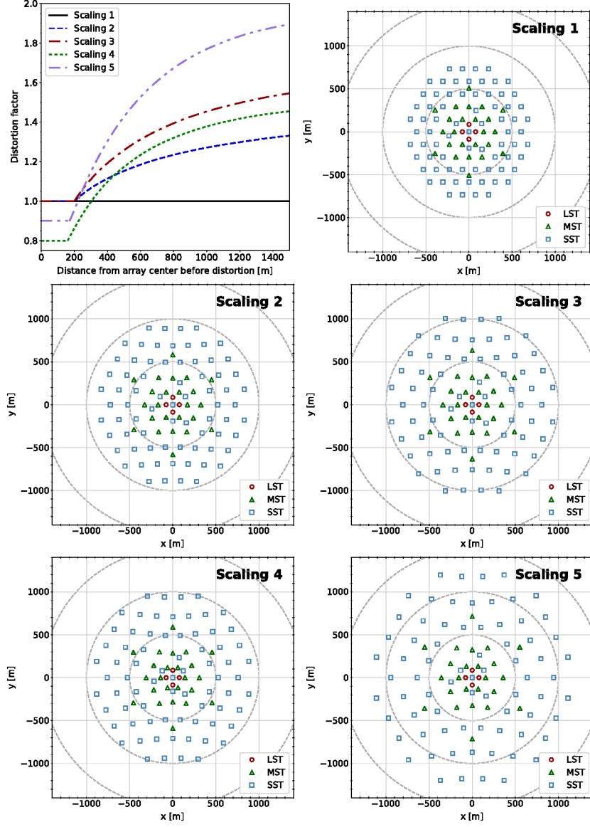
Figure 2: Top-left : Radially-symmetric distortion factors for the five different scalings applied to the CTA-South layouts, as a function of the radial distance to the centre of the array before the applied transformation. Top-right to bottom-right : an example of the five resulting scaled layouts for one of the Paranal site candidates (“S1”). LST positions are indicated by red circles, MSTs by green triangles, and SSTs by blue squares. Taken from [21].
