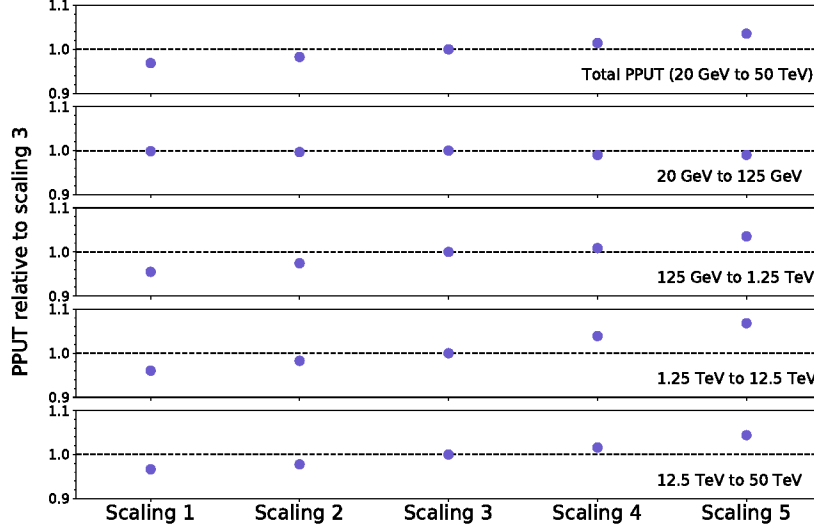
Figure 13: Relative PPUT values for the different scalings of the proposed layout for the northern site, all shown in Fig. 1, relative to the scaling 3.
