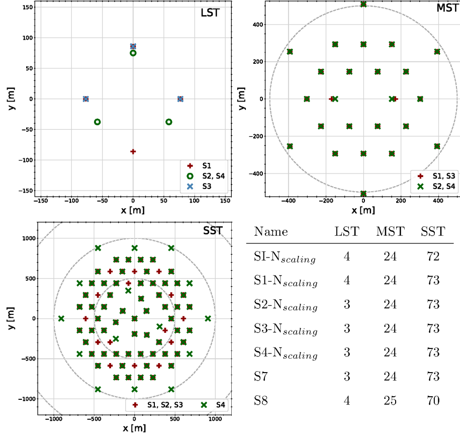
Figure 3: Simulated telescope positions for the different CTA-South array candidates. The positions of each telescope sub-system is shown separately for the arrays “S1” to “S4”. The table shows the number of telescopes per type for all layout candidates.
