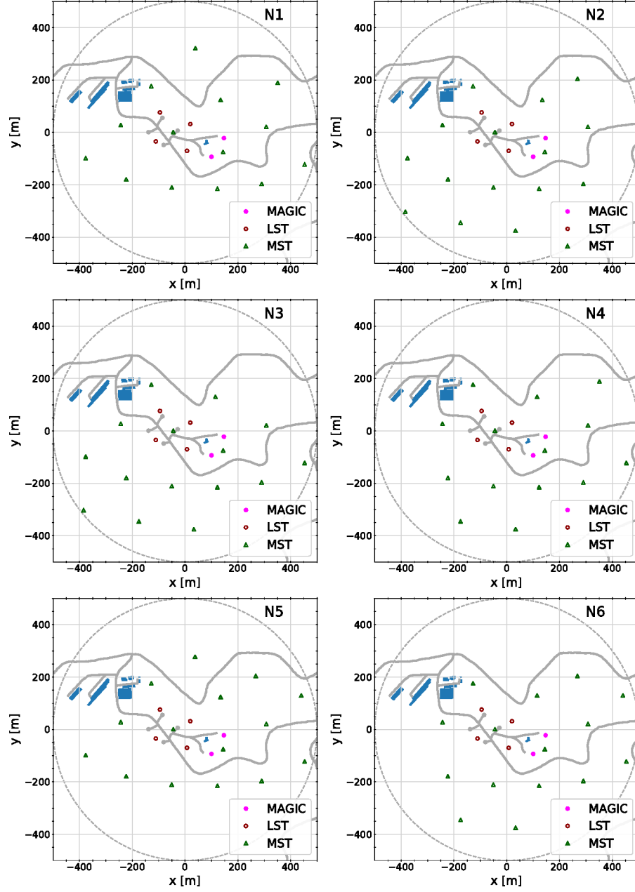
Figure 14: Several layouts proposed as baseline arrays for the northern site, together with the position of buildings, roads, and the two MAGIC telescopes. The orography constraints are not shown. The layouts share the LST positions and roughly the same inter-telescope distances between MSTs.
