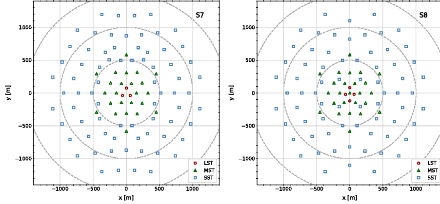
Figure 12: The best performing layouts from Fig. 11: “S7”, on the left, and the proposed baseline layout for the southern site, “S8”, on the right.
