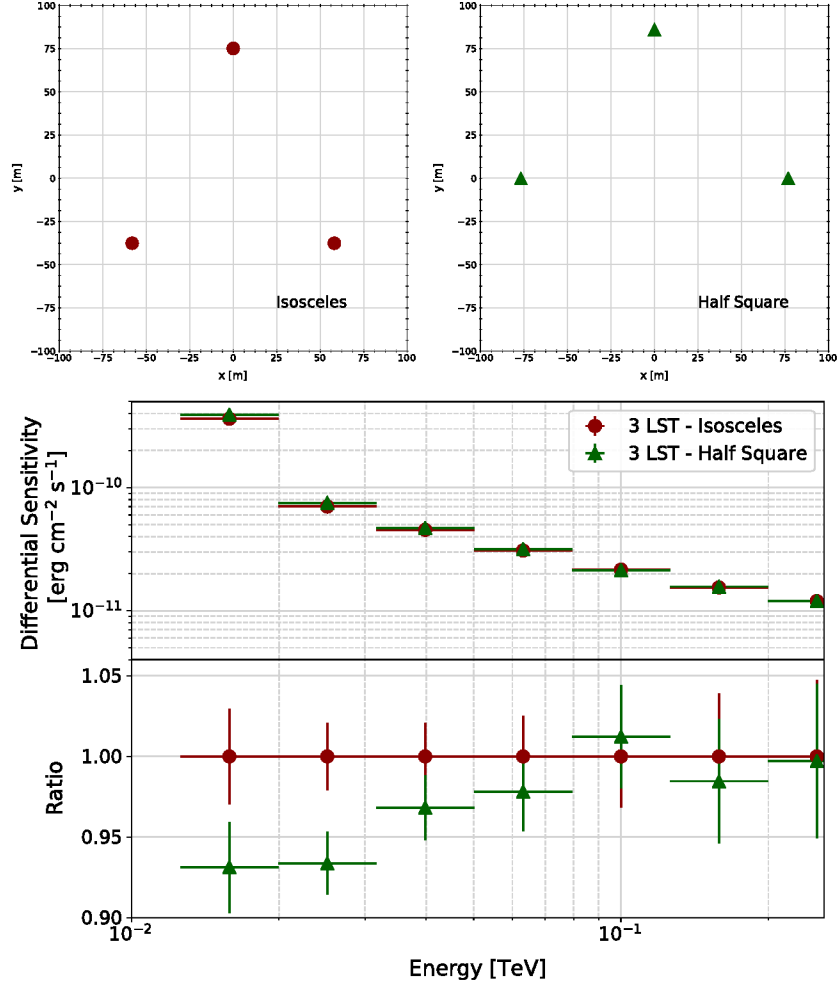
Figure 6: Differential sensitivity and differential sensitivity ratio as a function of energy for two configurations of three LSTs with equal area ( bottom ): arranged as half a square of 115 m on a side ( top right ) or an isosceles triangle with two 127 m sides (close to equilateral, top left ). The layouts are slightly stretched in the north-south direction and compressed in the east-west direction, as explained in section 2.1. The ratio is calculated so that higher values correspond to better sensitivity.
