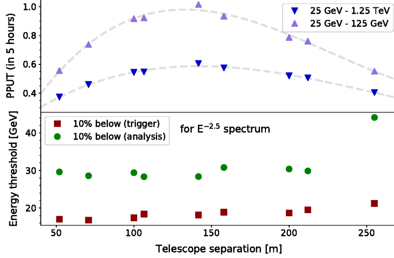
Figure 8: Performance (expressed in terms of PPUT, see text) and energy threshold of pairs of LSTs as a function of their separation. PPUT values are calculated from the average of the Aar and the two Leoncito site candidates (with an average altitude close to that of the Paranal site) and are also averaged over observations pointing towards north and south. The upper panel shows PPUT values in the energy ranges of 25 GeV to 125 GeV and 25 GeV to 1.25 TeV; the lower panel shows the calculated energy threshold by using the true energy value that leaves 10% of the events below the cut value (after either the trigger or the analysis) [37]. The performance is derived from the baseline analysis described in [12].
