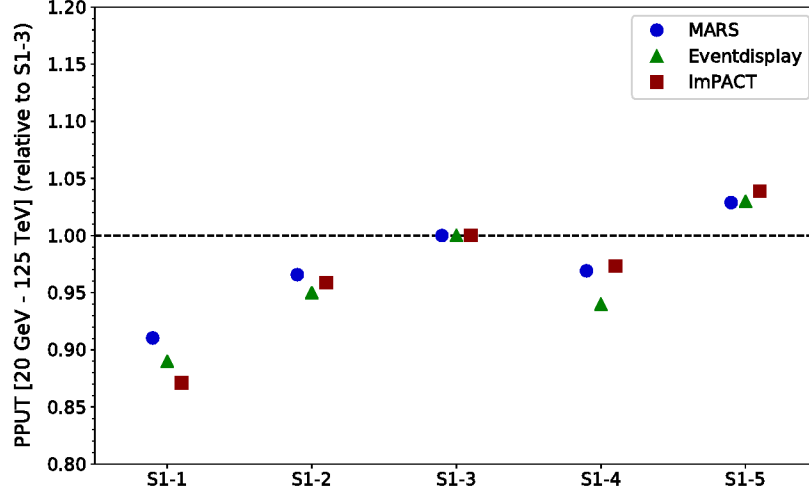
Figure 4: Comparison of performance (expressed in terms of PPUT, see text) of a range of simulated array layouts for three different analysis chains, relative to the PPUT value attained by each of them on the “S1-3” layout. The five layouts are presented in Fig. 2. The symbols shown in the legend indicate the various analysis chains.
