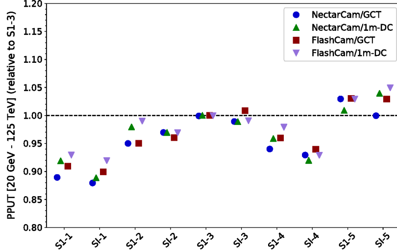
Figure 5: Comparison of performance (expressed in terms of PPUT, see text) of a range of simulated CTA-South array layouts for different combinations of telescope model configurations, each relative to the “S1-3” layout. The different “S1” layout scalings are pictured in Fig. 2, while the “ST” layouts are described in section 3.2. The symbols shown in the legend indicate the various telescope configurations.
