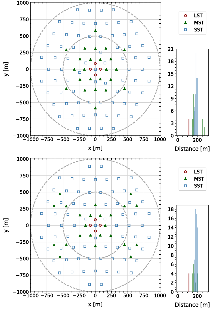
Figure 9: Layouts with different MST patterns: “S1” ( top ), with a strictly hexagonal pattern and “SI” ( bottom ), with four islands and a hexagonal core. The LST positioning in the two cases is the same, while the SSTs have been rearranged. Both layouts correspond to their scaling 2 variation. The distance of each telescope to its nearest neighbour of the same type is shown on the right.
