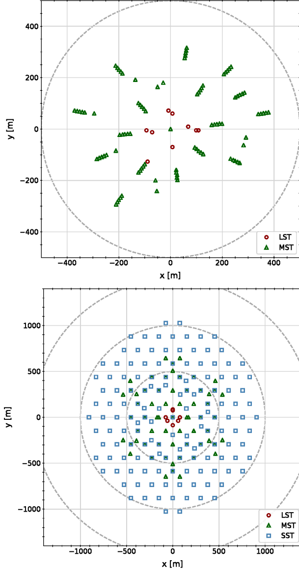
Figure 1: Simulated telescope positions within the third large-scale MC production (see section 2 for details). Top : La Palma telescope positions including all radially-scaled MST layouts. The available positions are restricted by the site topography, buildings and roads. Bottom : Paranal telescope positions before applying any radially-symmetric transformation (scaling number 1). LST positions are indicated by red circles, MSTs by green triangles, and SSTs by blue squares.
