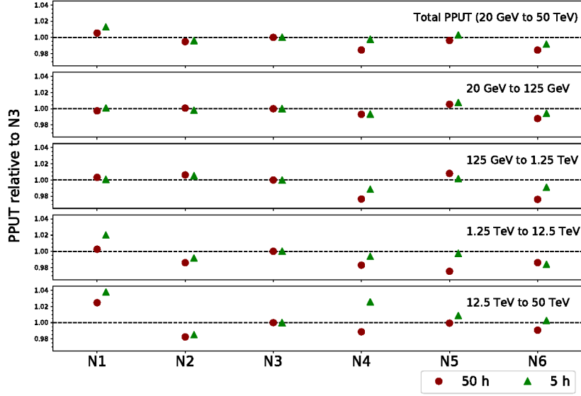
Figure 15: Relative PPUT values for several different candidates for the northern layout, relative to “N3”. The differences between the layouts are less than 5%.
