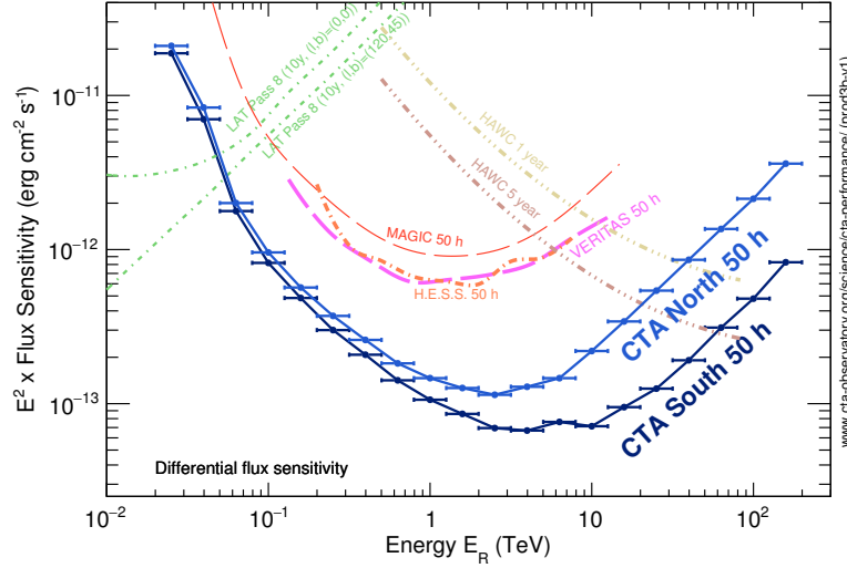
Figure 16: CTA differential sensitivity (multiplied by energy squared) compared to those of present day instruments (from [38]): Fermi-LAT [39], MAGIC [40, 41], H.E.S.S. [42], VERITAS [43], and HAWC [44]
