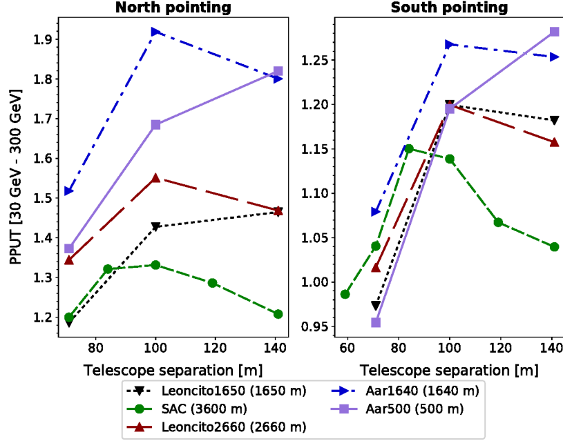
Figure 7: Performance (expressed in terms of PPUT, see text) of LST squared layouts of different sizes located at different CTA-South candidate sites ( left : observations towards north, right : observations towards south), in the energy range 30 to 300 GeV, using the baseline analysis described in [12].
