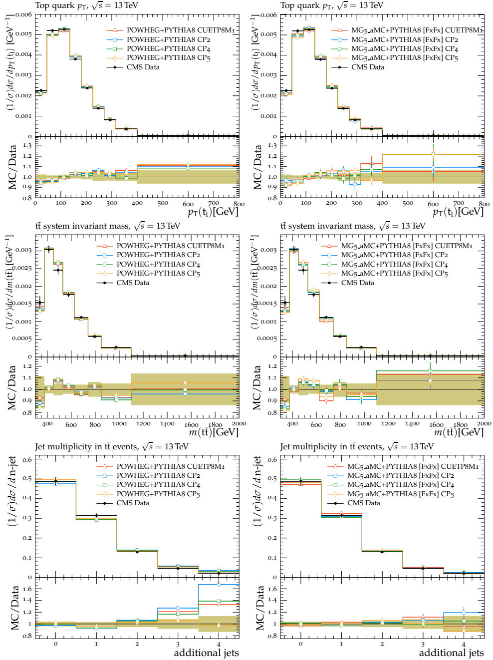
Figure 16: The normalized t\bar{t} cross section in the lepton+jets channel, as a function of the transverse momentum of the top quark for leptonically decaying top quarks ( t_\ell ) (upper), the invariant mass of the t\bar{t} system, m(t\bar{t}) (middle), and in bins of number of additional jets (lower) from CMS \sqrt{s} = 13 TeV analysis [66]. The data are compared with the predictions of POWHEG (left) and MG5_aMC [FxFx] (right). In both cases, the PS simulation is done with the PYTHIA8 tunes CUETP8M1, CP2, CP4, or CP5. Tunes CP1 and CP3 are not shown in the plot but present a similar behaviour as, respectively, tunes CP2 and CP4. The ratios of simulations to the data (MC/Data) are also shown, where the shaded band indicates the total experimental uncertainty in the data. Vertical lines drawn on the data points refer to the total uncertainty in the data. Vertical lines drawn on the MC points refer to the statistical uncertainty in the predictions. Horizontal bars indicate the associated bin width.
