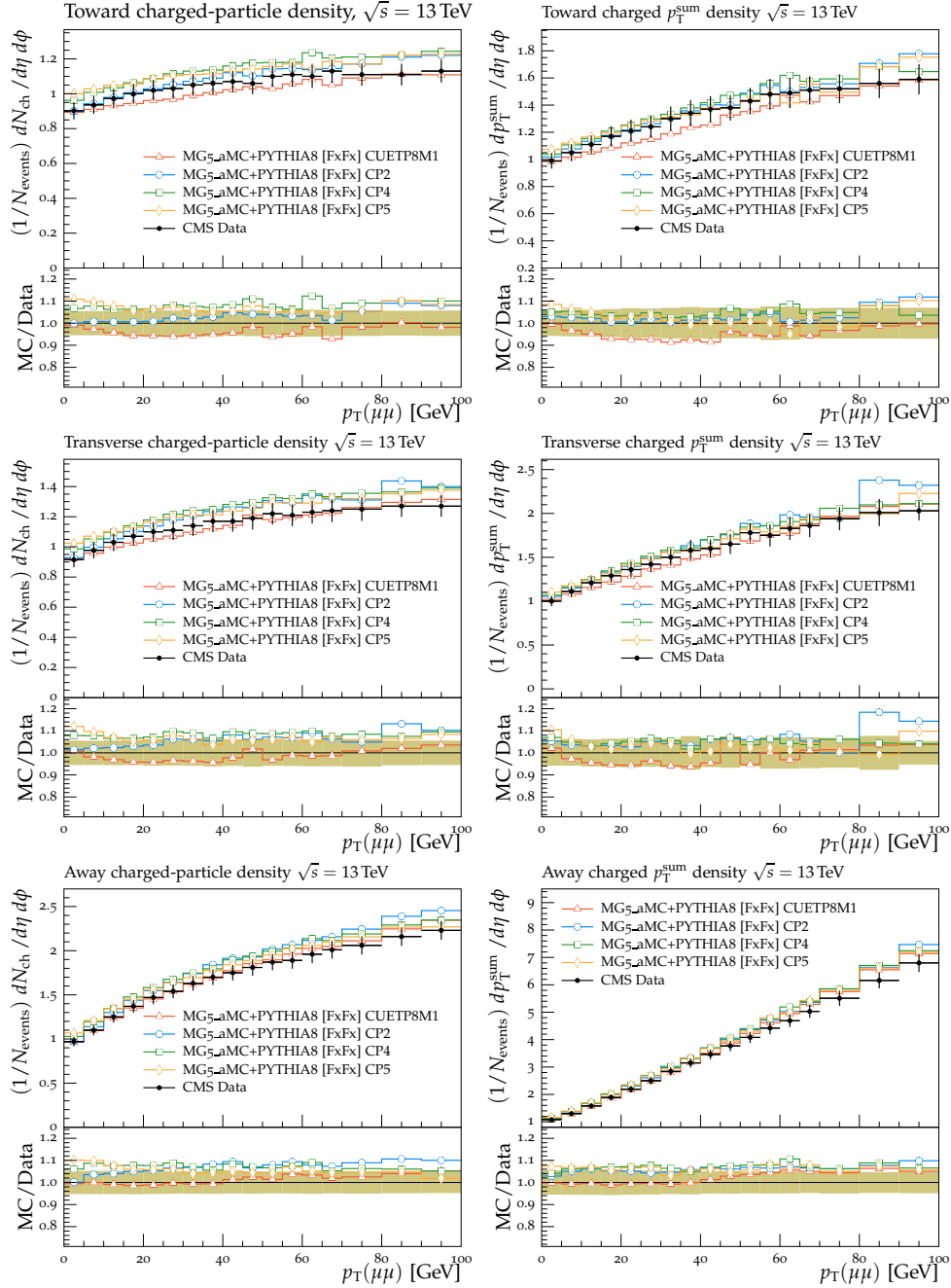
Figure 17: The charged-particle multiplicity (left) and p_T^{\text{sum}} (right) in the toward (upper), transverse (middle), and away (lower) regions measured as a function of the Z boson p_T in Drell–Yan events at \sqrt{s} = 13 TeV [21], and compared with the predictions obtained by an inclusive NLO ME calculated by MG5_aMC, interfaced to the UE simulation of PYTHIA8 with the CUETP8M1, CP2, CP4, and CP5 tunes. Tunes CP1 and CP3 are not shown in the plot but present a similar behaviour as, respectively, tunes CP2 and CP4. The ratios of simulations to the data (MC/Data) are also shown, where the shaded band indicates the total experimental uncertainty of the data. Vertical lines drawn on the data points refer to the total uncertainty in the data. Vertical lines drawn on the MC points refer to the statistical uncertainty in the predictions. Horizontal bars indicate the associated bin width.
