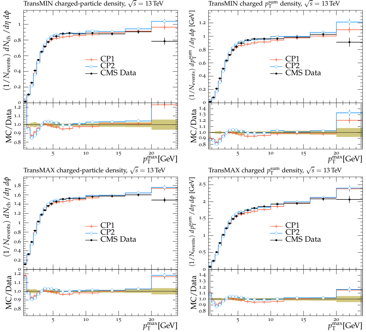
Figure 3: The transMIN (upper left) charged-particle and (upper right) charged p_T^{\text{sum}} densities and the transMAX (lower left) charged-particle and (lower right) charged p_T^{\text{sum}} densities, as a function of the transverse momentum of the leading charged particle, p_T^{\text{max}} , from the CMS \sqrt{s} = 13 TeV analysis [16]. Charged hadrons are measured with p_T > 0.5 GeV in |\eta| < 2.0 . The transMIN densities are more sensitive to the MPI, whereas the transMAX densities are more sensitive to ISR and FSR. The data are compared with the CMS PYTHIA8 LO-PDF tunes CP1 and CP2. The ratios of the simulations to the data (MC/Data) are also shown, where the shaded band indicates the total experimental uncertainty in the data. Vertical lines drawn on the data points refer to the total uncertainty in the data. Vertical lines drawn on the MC points refer to the statistical uncertainty in the predictions. Horizontal bars indicate the associated bin width.
