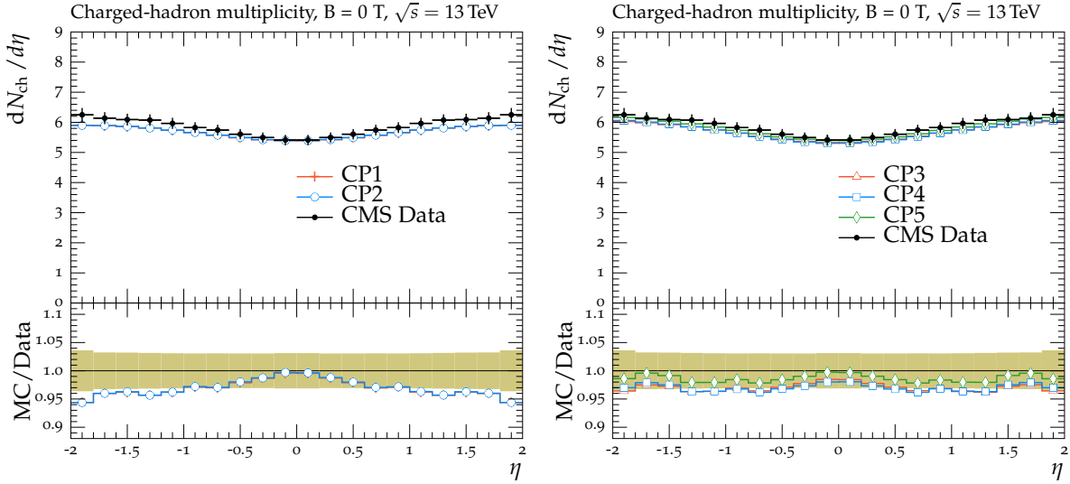
Figure 9: The pseudorapidity distribution of charged hadrons measured in |\eta| < 2 for an inclusive selection in inelastic proton-proton collisions, with zero magnetic field strength ( B = 0 T), from the CMS \sqrt{s} = 13 TeV analysis [18]. The data are compared with (left) the CMS PYTHIA8 LO-PDF tunes CP1 and CP2, and with (right) the CMS PYTHIA8 NLO-PDF tune CP3 and the CMS PYTHIA8 NNLO-PDF tunes CP4 and CP5. The ratios of simulations to the data (MC/Data) are also shown, where the shaded band indicates the total experimental uncertainty in the data. Vertical lines drawn on the data points refer to the total uncertainty in the data. Vertical lines drawn on the MC points refer to the statistical uncertainty in the predictions. Horizontal bars indicate the associated bin width.
