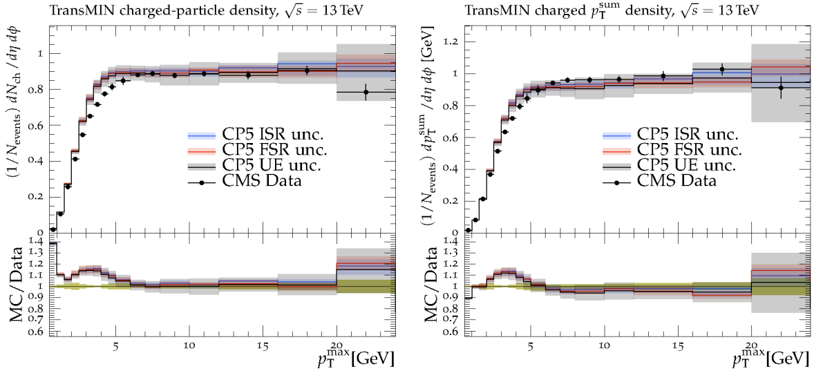
Figure 21: The variations allowed by the CP5 tune when \alpha_S^{\text{ISR}}(m_Z) (blue band) and \alpha_S^{\text{FSR}}(m_Z) (red band) are left free in the fit for charged-particle (left) and charged p_T^{\text{sum}} (right) density in the transMIN region at \sqrt{s} = 13 TeV. Vertical lines drawn on the data points refer to the total uncertainty in the data. The grey band represents the total UE uncertainty for the tune CP5. Horizontal bars indicate the associated bin width.
