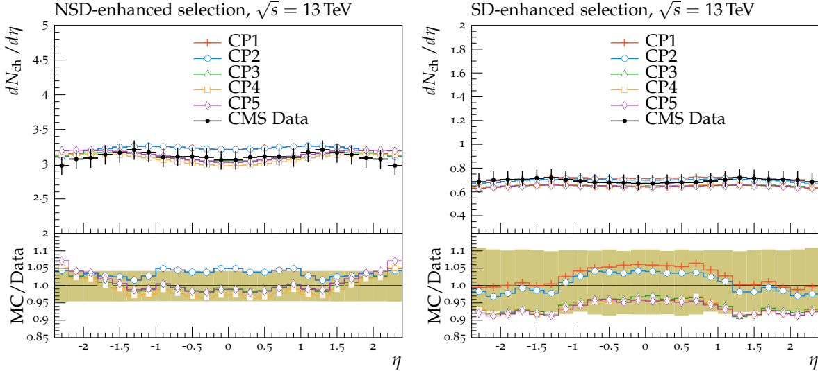
Figure 10: The pseudorapidity distribution ( p_T > 0.5 \text{ GeV} , |\eta| < 2.4 ) for (left) the NSD-enhanced and (right) the SD-enhanced event selection of charged particles in inelastic proton-proton collisions, from the CMS \sqrt{s} = 13 \text{ TeV} analysis [24]. The data are compared with the CMS PYTHIA8 LO-PDF tunes CP1 and CP2, the CMS PYTHIA8 NLO-PDF tune CP3, and the CMS PYTHIA8 NNLO-PDF tunes CP4 and CP5. The ratio of the simulations to the data (MC/Data) is also shown, where the shaded band indicates the total experimental uncertainty in the data. Vertical lines drawn on the data points refer to the total uncertainty in the data. Vertical lines drawn on the MC points refer to the statistical uncertainty in the predictions. Horizontal bars indicate the associated bin width.
