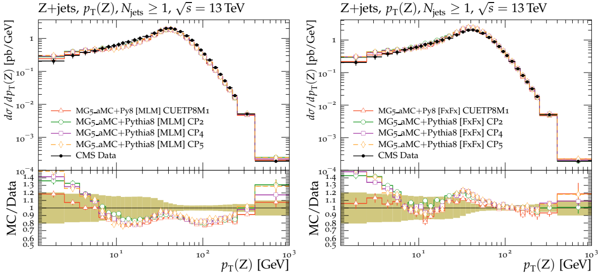
Figure 20: Comparison with the measurement [67] of the p_T(Z) predicted by MG5_aMC + PYTHIA8 with k_T -MLM merging (left) and FxFx merging (right) for the different tunes. Tunes CP1 and CP3 are not shown in the plot but they present a similar behaviour as tunes CP2 and CP4, respectively. The ratios of simulations to the data (MC/Data) are also shown, where the shaded band indicates the total experimental uncertainty in data. Vertical lines drawn on the data points refer to the total uncertainty in the data. Vertical lines drawn on the MC points refer to the statistical uncertainty in the predictions. Horizontal bars indicate the associated bin width.
