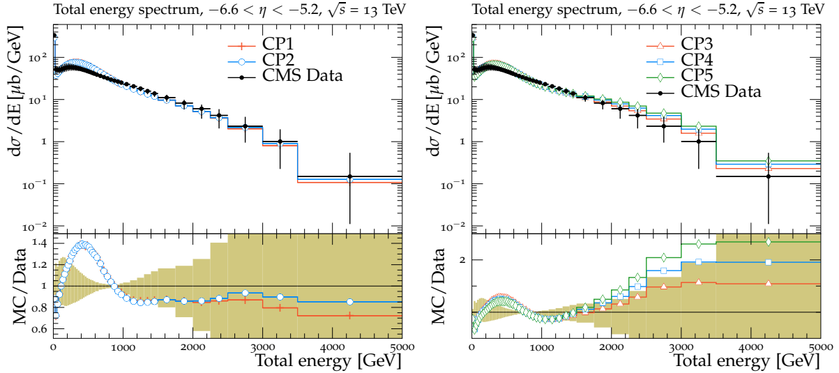
Figure 13: The total energy spectrum measured in the pseudorapidity interval -6.6 < \eta < -5.2 , from the CMS \sqrt{s} = 13 TeV analysis [47]. The data are compared with (left) the CMS PYTHIA8 LO-PDF tunes CP1 and CP2, and with (right) the CMS PYTHIA8 NLO-PDF tune CP3 and the CMS PYTHIA8 NNLO-PDF tunes CP4 and CP5. The ratio of the simulations to the data (MC/Data) is also shown, where the shaded band indicates the total experimental uncertainty in the data. Vertical lines drawn on the data points refer to the total uncertainty in the data. Vertical lines drawn on the MC points refer to the statistical uncertainty in the predictions. Horizontal bars indicate the associated bin width.
