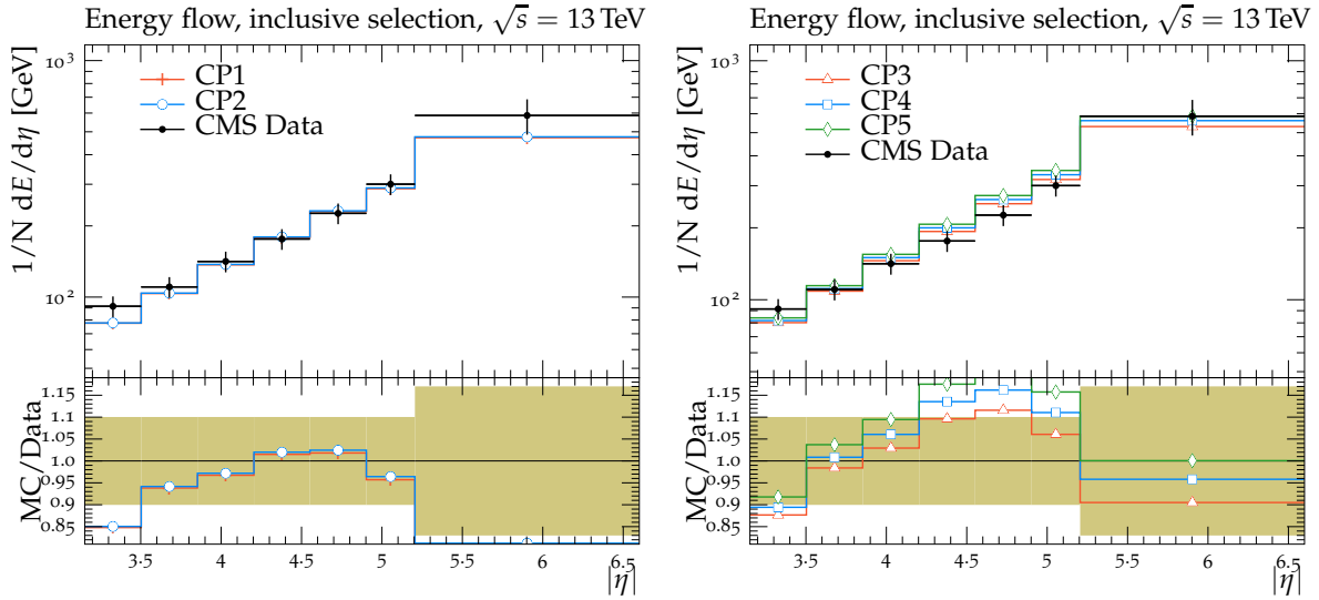
Figure 12: The energy flow measured in an inclusive selection as a function of pseudorapidity, from the CMS \sqrt{s} = 13 TeV analysis [45]. The data are compared with (left) the CMS PYTHIA8 LO-PDF tunes CP1 and CP2, and with (right) the CMS PYTHIA8 NLO-PDF tune CP3 and the CMS PYTHIA8 NNLO-PDF tunes CP4 and CP5. The ratio of the simulations to the data (MC/Data) is also shown, where the shaded band indicates the total experimental uncertainty in the data. Vertical lines drawn on the data points refer to the total uncertainty in the data. Vertical lines drawn on the MC points refer to the statistical uncertainty in the predictions. Horizontal bars indicate the associated bin width.
