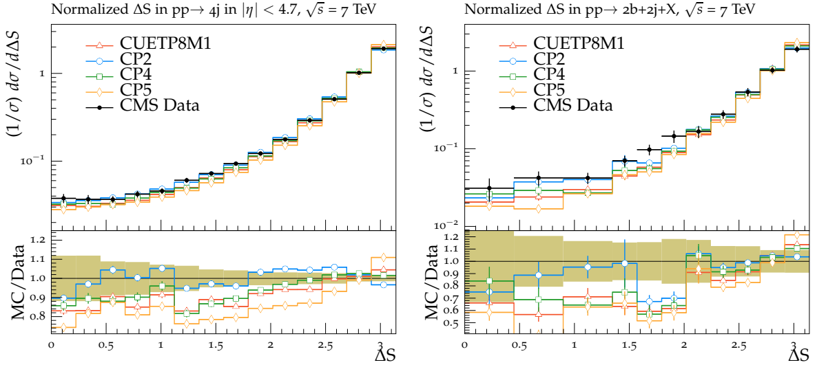
Figure 15: The correlation observable \Delta S measured in 4j (left) and 2b2j (right) production, compared to predictions of PYTHIA8 tunes CUETP8M1, CP2, CP4, and CP5, from the CMS \sqrt{s} = 7 TeV analyses [59, 61]. Tunes CP1 and CP3 are not shown in the plot but show a similar behaviour as, respectively, tunes CP2 and CP4. The ratios of simulations to the data (MC/Data) are also shown, where the shaded band indicates the total experimental uncertainty in the data. Vertical lines drawn on the data points refer to the total uncertainty in the data. Vertical lines drawn on the MC points refer to the statistical uncertainty in the predictions. Horizontal bars indicate the associated bin width.
