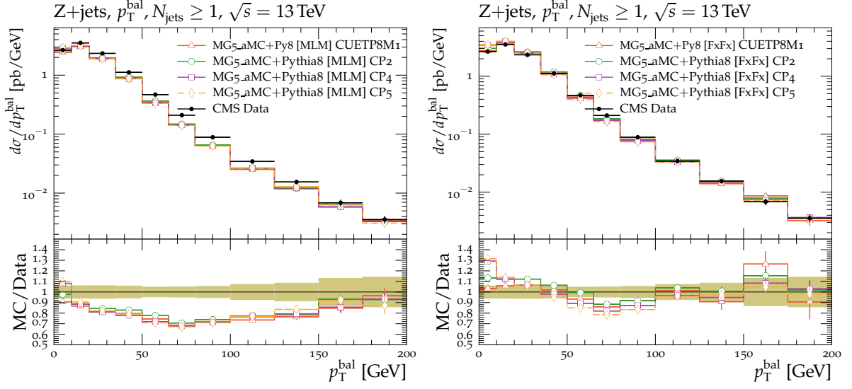
Figure 19: Comparison with the measurement [67] of the p_T balance predicted by MG5_aMC + PYTHIA8 with k_T -MLM merging (left) and FxFx merging (right) for the different tunes for events with at least one jet. Tunes CP1 and CP3 are not shown in the plot but they present a similar behaviour as tunes CP2 and CP4, respectively. The ratios of simulations to the data (MC/Data) are also shown, where the shaded band indicates the total experimental uncertainty in the data. Vertical lines drawn on the data points refer to the total uncertainty in the data. Vertical lines drawn on the MC points refer to the statistical uncertainty in the predictions. Horizontal bars indicate the associated bin width.
