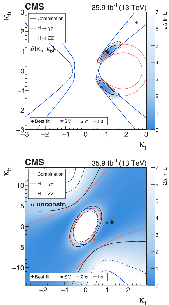
Fig. 10. Simultaneous fit to data for \kappa_t and \kappa_b , assuming a coupling dependence of the branching fractions (upper) and the branching fractions implemented as nuisance parameters with no prior constraint (lower). The one standard deviation contour is drawn for the combination ( H \rightarrow \gamma\gamma , H \rightarrow ZZ , and H \rightarrow b\bar{b} ), the H \rightarrow \gamma\gamma channel, and the H \rightarrow ZZ channel in black, red, and blue, respectively. For the combination the two standard deviation contour is drawn as a black dashed line, and the shading indicates the negative log-likelihood, with the scale shown on the right hand side of the plots.
