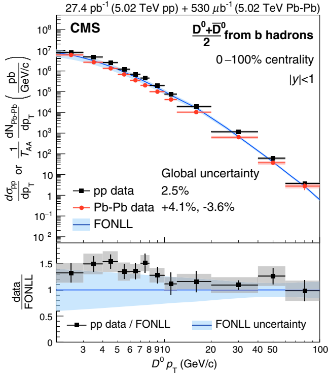
FIG. 2. Upper panel: B \rightarrow D^0 p_T -differential cross section in pp collisions and invariant yield in Pb-Pb collisions normalized with T_{AA} , at \sqrt{s_{NN}} = 5.02 TeV. The vertical bands around the data points represent the bin-by-bin systematic uncertainties. Uncertainties are smaller than the symbols in most cases. The cross section in pp collisions is compared to FONLL calculations [33]. Lower panel: The data/FONLL ratio for the B \rightarrow D^0 p_T spectra in pp collisions.
